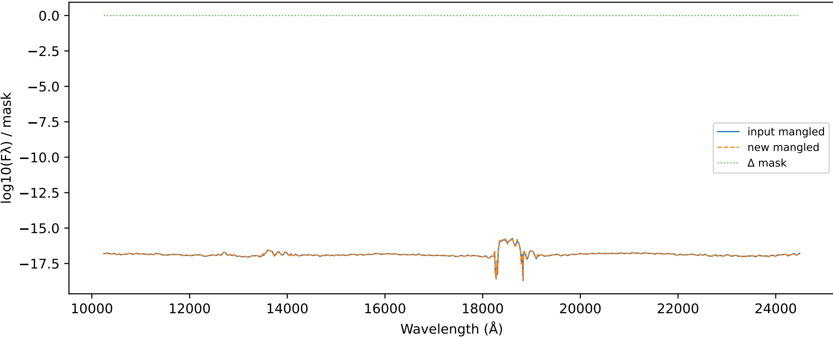
Mangle delta MJD 57991.0000 NIR_AT2017gfo_ENGRAVE_v1.0_XSHOOTER_MJD-57991.000001_Phase+8.40d.dat
