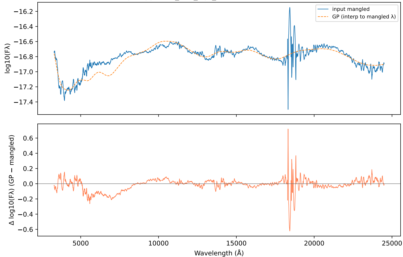
Group suggested_007_mjd_57990.0000 MJD 57990.0000
