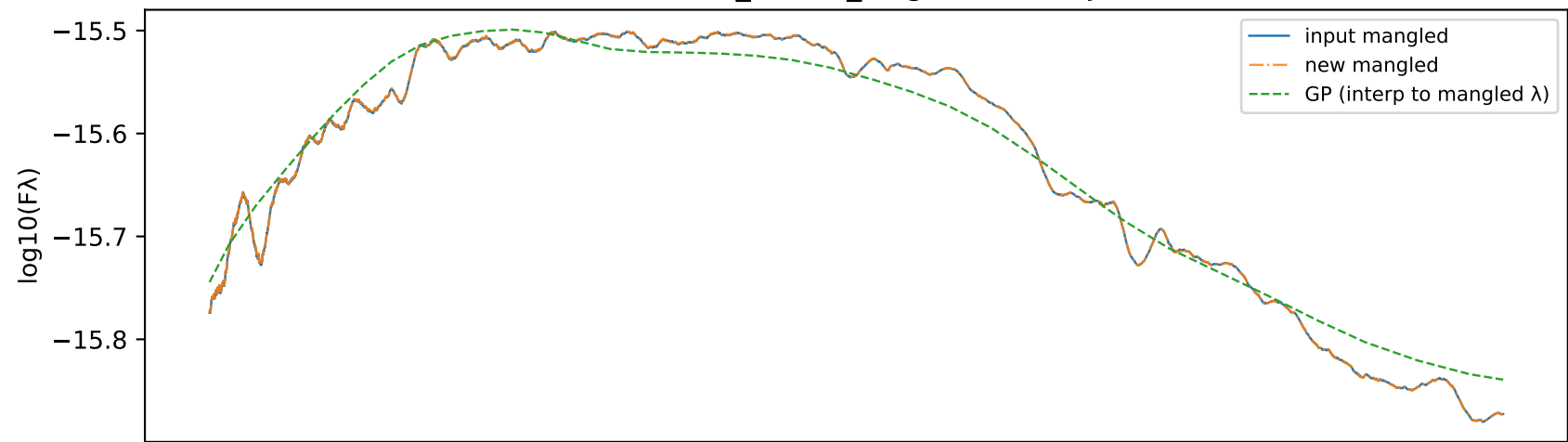
Individual 57984.0484_LDSS3_Magellan.dat MJD 57984.0484
