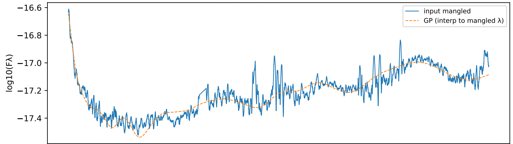
Group suggested_010_mjd_57993.0000 MJD 57993.0000
