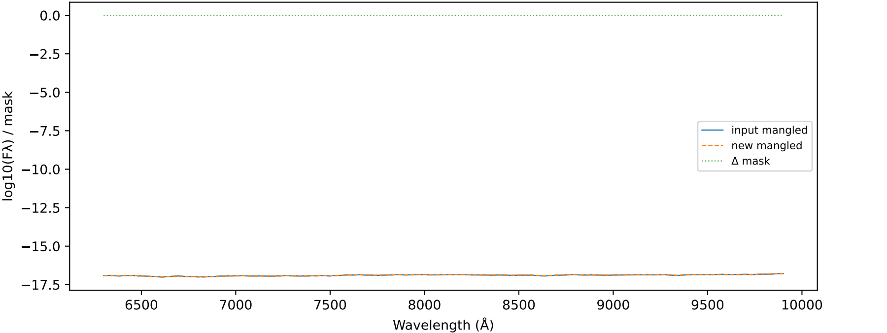
Mangle delta MJD 57991.0000 VIS_AT2017gfo_ENGRAVE_v1.0_XSHOOTER_MJD-57991.000003_Phase+8.40d.dat
