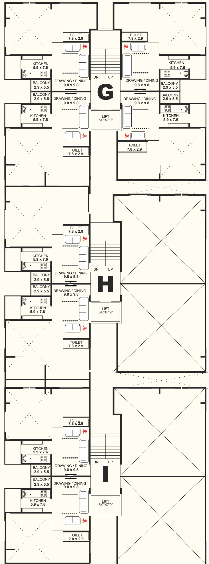
Typical Floor Plan (F.F.)
