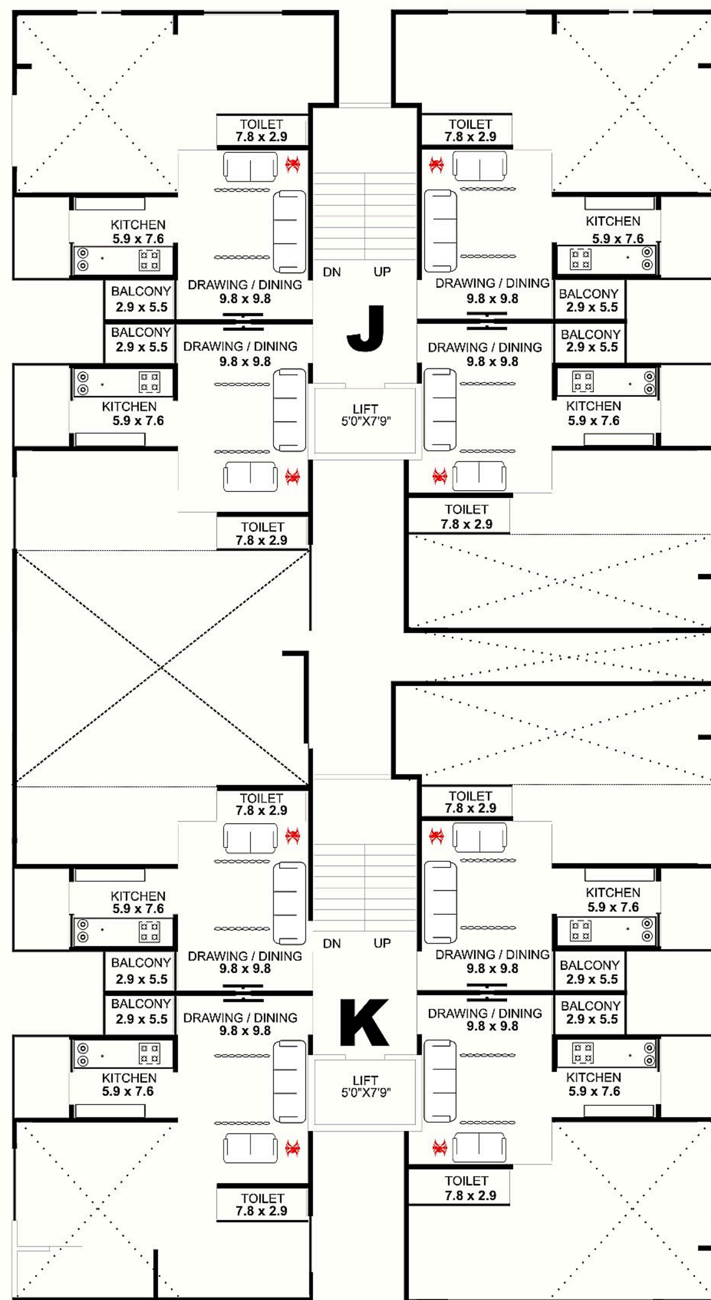
Typical Floor Plan (F.F.)
