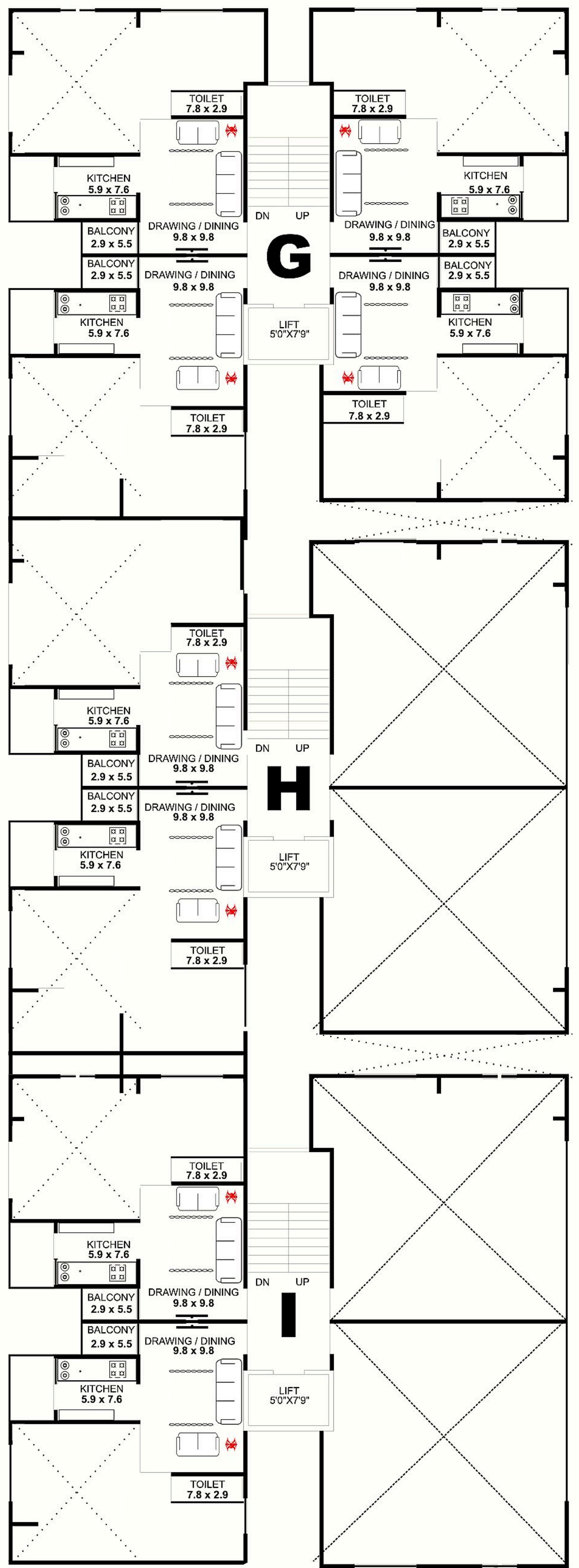
Typical Floor Plan (F.F.)
