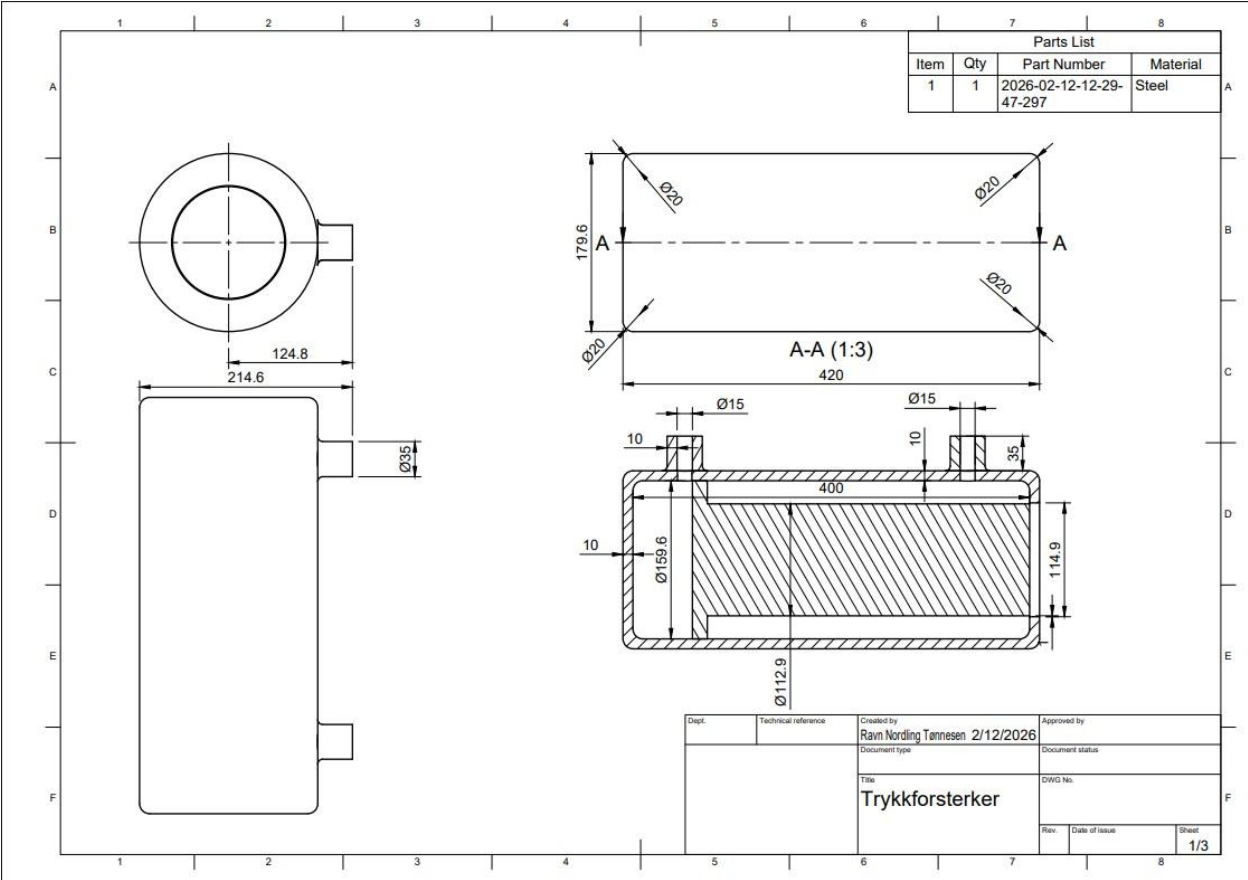
A simple hydraulic pressurizer(Full system not drawn)
