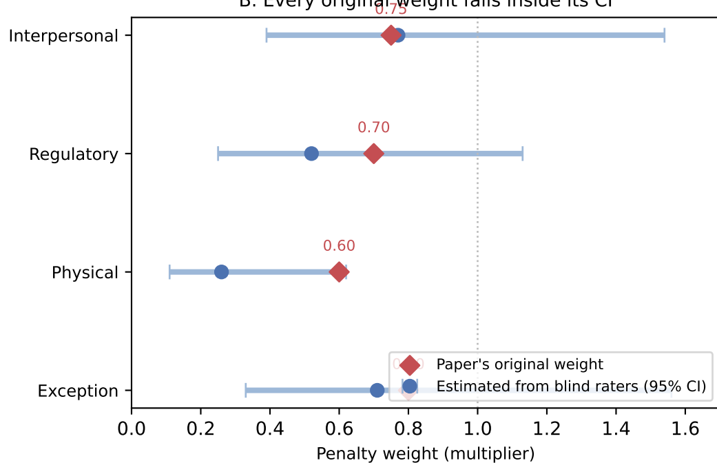
B. Every original weight falls inside its CI
