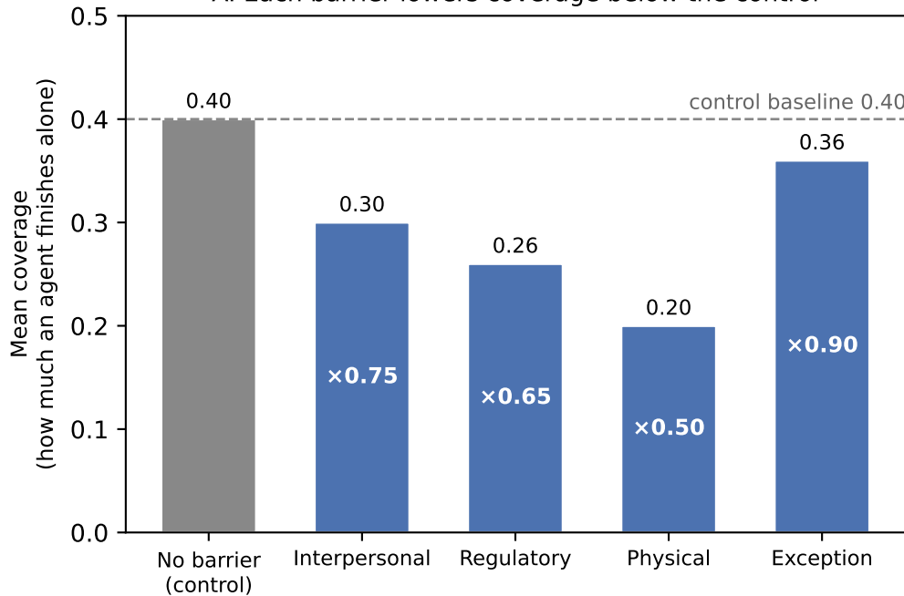
A. Each barrier lowers coverage below the control
