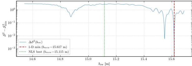
Lab brute-force step 1: 1-D sweep of \mathcal{S}^2 vs b_{ew}
