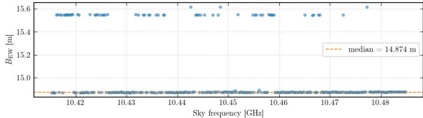
FFT baseline per channel (all chips pooled)
