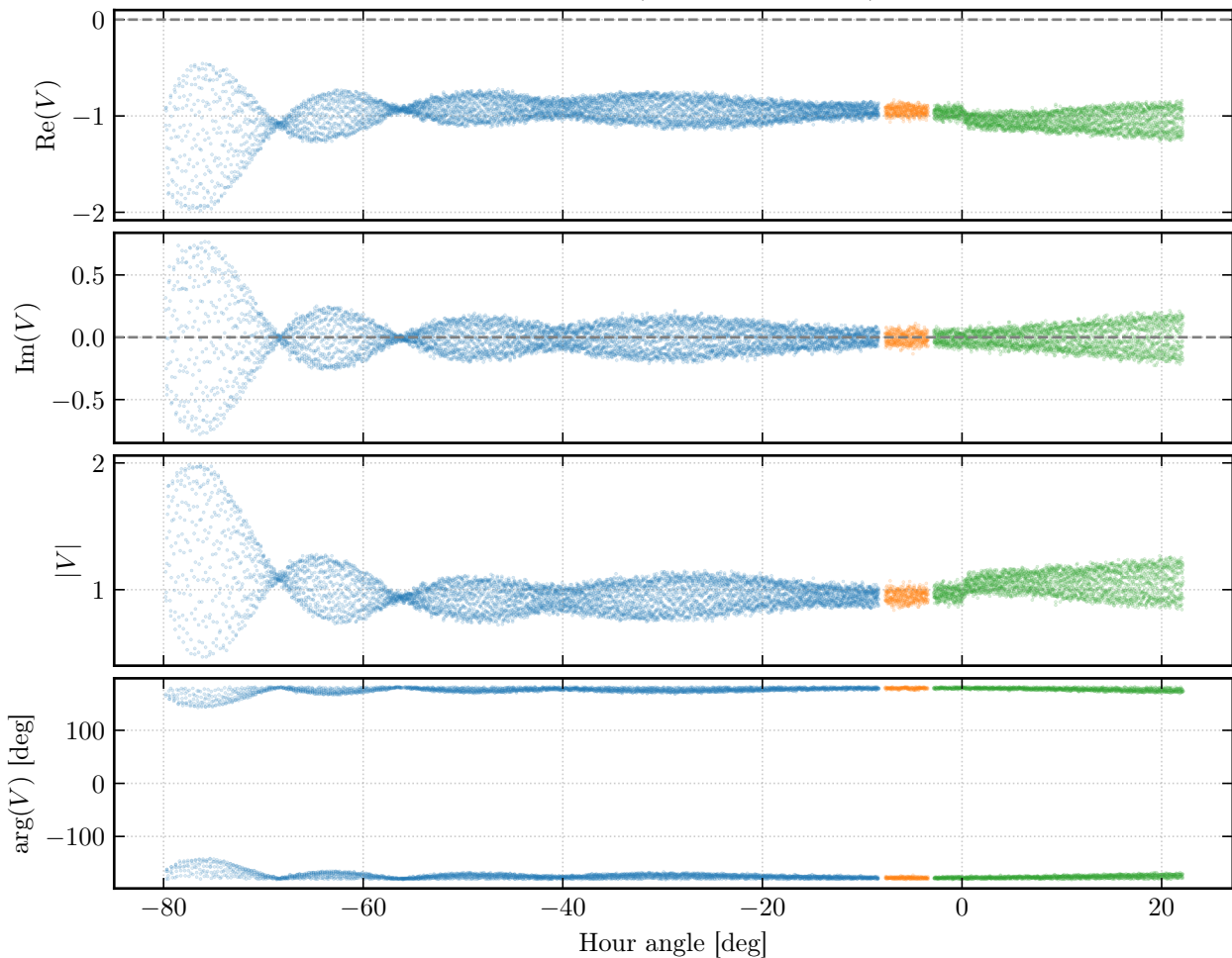
Raw visibility (ch 655, 10.450 GHz)
