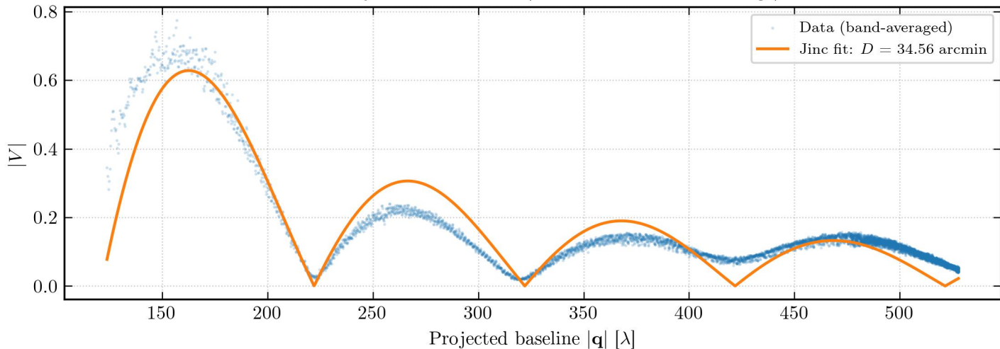
Standard jinc fit with R free (constrained to extrema range)
