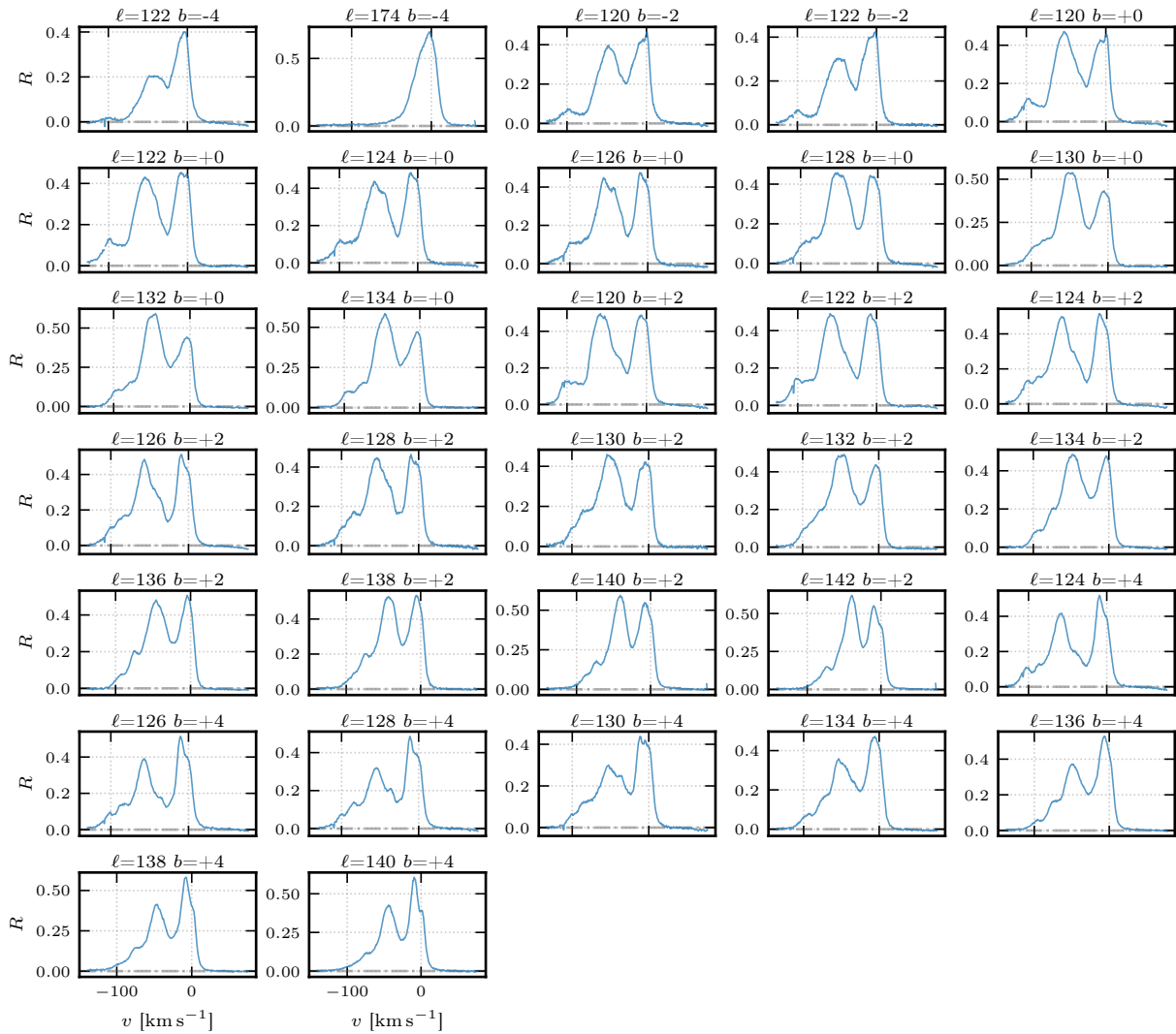
session_011 – 32 pointings (post pair filter + QA, LSR frame)
