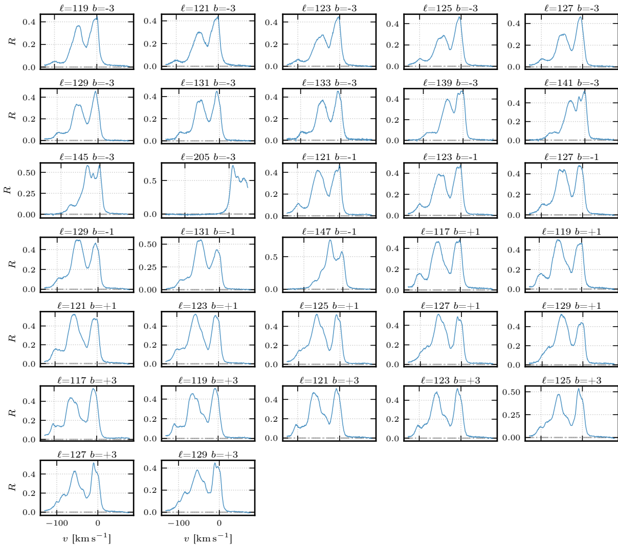
session_034 – 32 pointings (post pair filter + QA, LSR frame)
