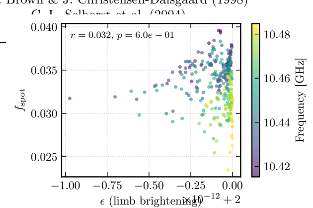
Fig. 14.— Limb-brightening coefficient \varepsilon versus sunspot floor f across all 285 channels. The Pearson correlation coefficient quantifies the partial degeneracy between these parameters: both raise the visibility near the Bessel nulls, and the fit trades between them.
