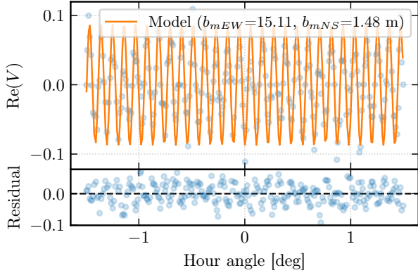
Fig. 10.— Recovered fringe pattern near transit ( |h| \leq 1.5^\circ ) from the windowed grid search. Top : observed \text{Re}(V) (scatter) and best-fit sinusoidal model (solid), illustrating the rapid fringe oscillation resolved by the interferometer. Bottom : fit residuals.
