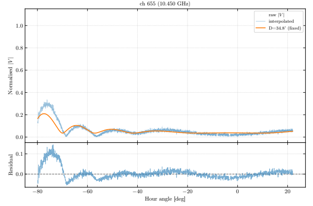
Fig. 12.— Three-parameter limb-brightened disk + sunspot floor fit at a representative channel. The data scatter shows |V| versus hour angle; the model curve includes both the jinc envelope and the sunspot floor.
