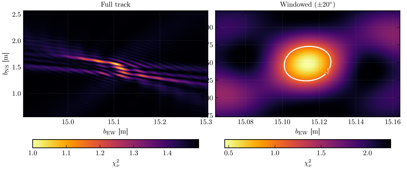
Fig. 9.— 2-D brute-force \chi^2_\nu grid search in the (b_{\text{ew}}, b_{\text{ns}}) plane. Left : Full-track search using all hour angles. Right : Windowed search restricted to |h| \leq 20^\circ around transit, suppressing Bessel-envelope bias. The 1\sigma confidence contour ( 2.30\times the minimum \chi^2_\nu ) is shown for illustration; adopted uncertainties come from the analytical curvature matrix. The windowed result ( b_{\text{ew}} = 15.114 m) is closer to the adopted baseline than the full-track grid ( b_{\text{ew}} = 15.103 m), consistent with a small systematic from the envelope modulation at large |h| .
