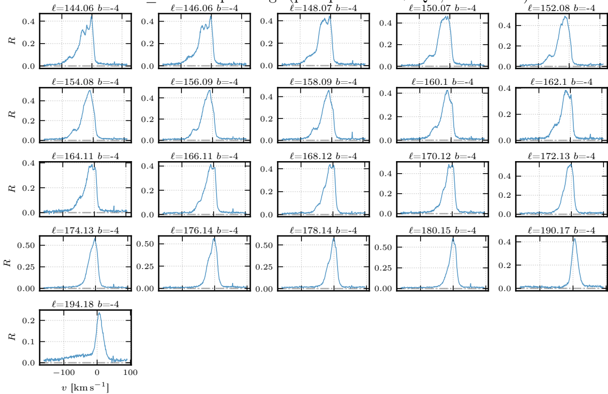
session_006 – 21 pointings (post pair filter + QA, LSR frame)
