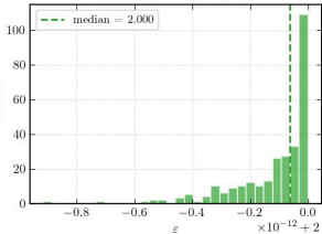
Limb-brightening coefficient
