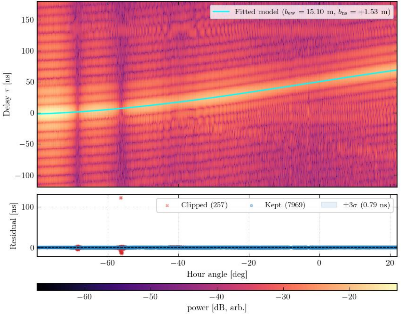
Fig. 8.— Delay spectrum versus hour angle (Method 3). Each point is the delay extracted from the IFFT of the cross-correlation spectrum V_{12}(\nu) at a single capture. The solid curve is the best-fit model \tau(h) = (b_{\text{ew}}/c) \cos \delta \sin h + (b_{\text{ns}}/c) \sin L \cos \delta \cos h + \tau_{\text{inst}} . The sinusoidal amplitude encodes b_{\text{ew}} ; the vertical offset at h = 0 is the effective cable delay \tau'_c .
