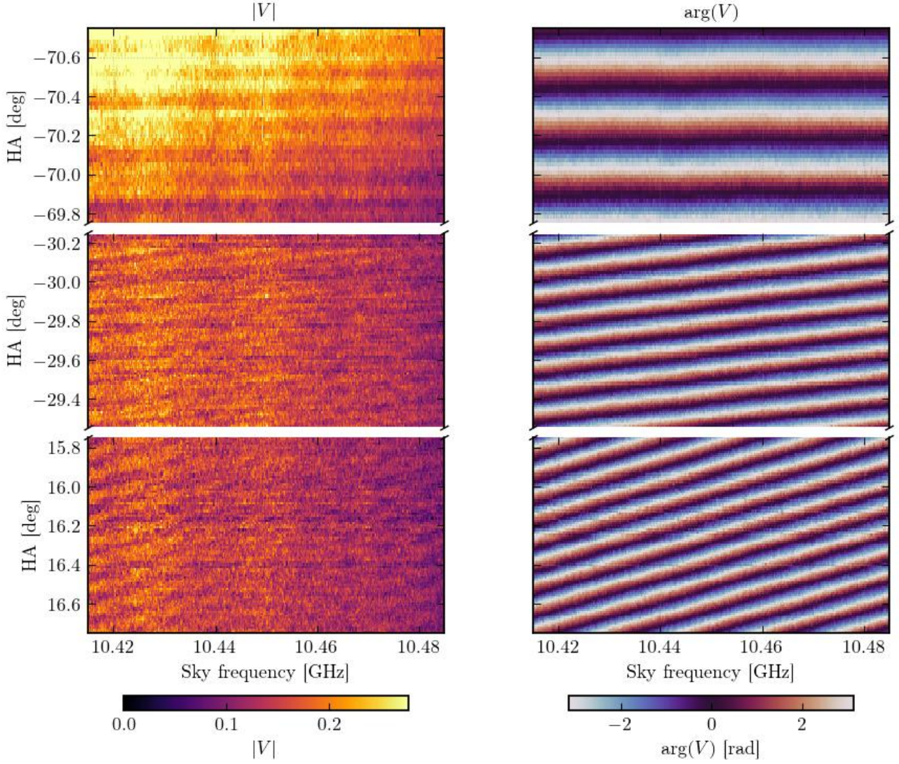
Fig. 5.— Waterfall plot of the DC-corrected visibility across the analysis band at three hour-angle windows. Left columns: Visibility amplitude |V(\nu, h)| . Right columns: Visibility phase \arg V(\nu, h) . The fringe pattern is tightly packed far from transit (high f_f ) and spreads out near transit (low f_f ). The phase slope across frequency at any given time encodes the geometric delay \tau_g(h) .
