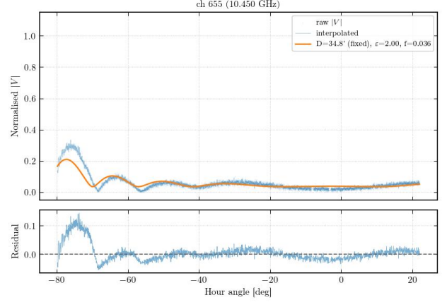
Fig. 15.— Three-parameter limb-brightened disk + sunspot floor fit at a representative channel. The data scatter shows |V| versus hour angle; the model curve includes both the jinc envelope and the sunspot floor.
