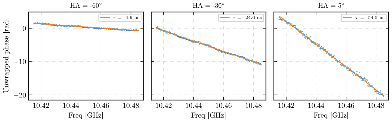
Fig. 7.— Phase slope across frequency at three hour angles. The linear slope encodes \tau_g directly; fitted delays agree with predictions to within a few nanoseconds.
