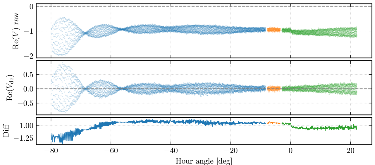
Fig. 4.— DC correction at a representative channel. Top : Raw \text{Re}(V) . Middle : DC-corrected \text{Re}(V_{\text{dc}}) , now symmetric about zero. Bottom : Difference (subtracted DC component). The amplitude drop near h \approx 0^\circ is likely due to a strong wind gust momentarily blowing a dish off-pointing.
