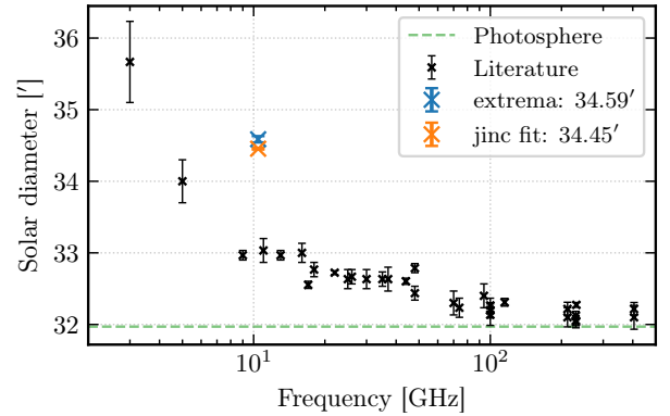
Fig. 12.— Solar diameter vs radio frequency. Black crosses show the literature compilation from F. Menezes et al. (2021) (Table 1), M. Marongiu et al. (2024), and references therein; our two measurements at 10.45 GHz are shown in colour. The dashed line marks the optical photospheric diameter. Our values sit \sim 5\% above the literature trend at comparable frequencies.
