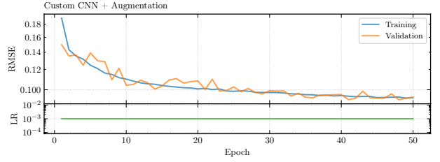
Fig. 24.— Custom CNN with rotation augmentation only (no LR scheduler, 50-epoch quick test, constant LR 10^{-3} ). The augmentation alone reaches val. RMSE \sim 0.0915 , already at the lab manual’s “good” target, and closes the train/val gap visibly compared to Figure 22. This is the augmentation-axis arm of the 2 \times 2 ablation; combining with the scheduler (Figure 25) adds a further \Delta\text{RMSE} \approx -0.0002 .
