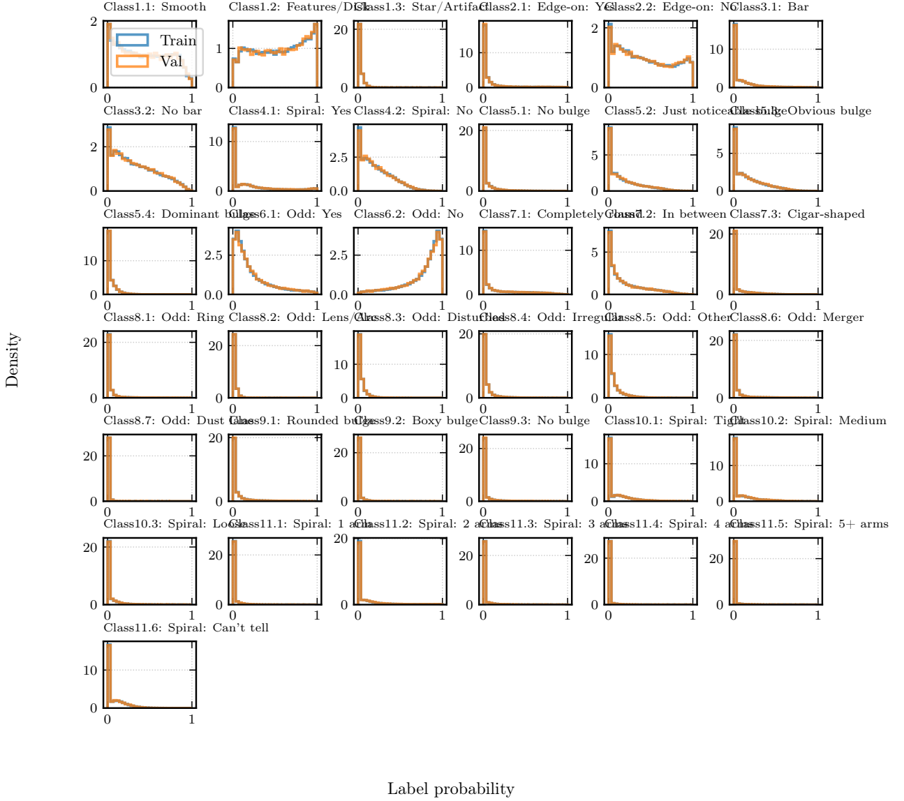
Fig. 17.— Per-label normalized histograms of the 80/20 train (blue) and validation (orange) split (seed 42). The two distributions overlap to within visible per-bin counting noise on every one of the 37 labels, confirming that the random split has not introduced any systematic label-prevalence drift between training and validation; per-label two-sample Kolmogorov–Smirnov tests cannot reject the null hypothesis of identical distributions at the \alpha = 0.05 level for any label.
