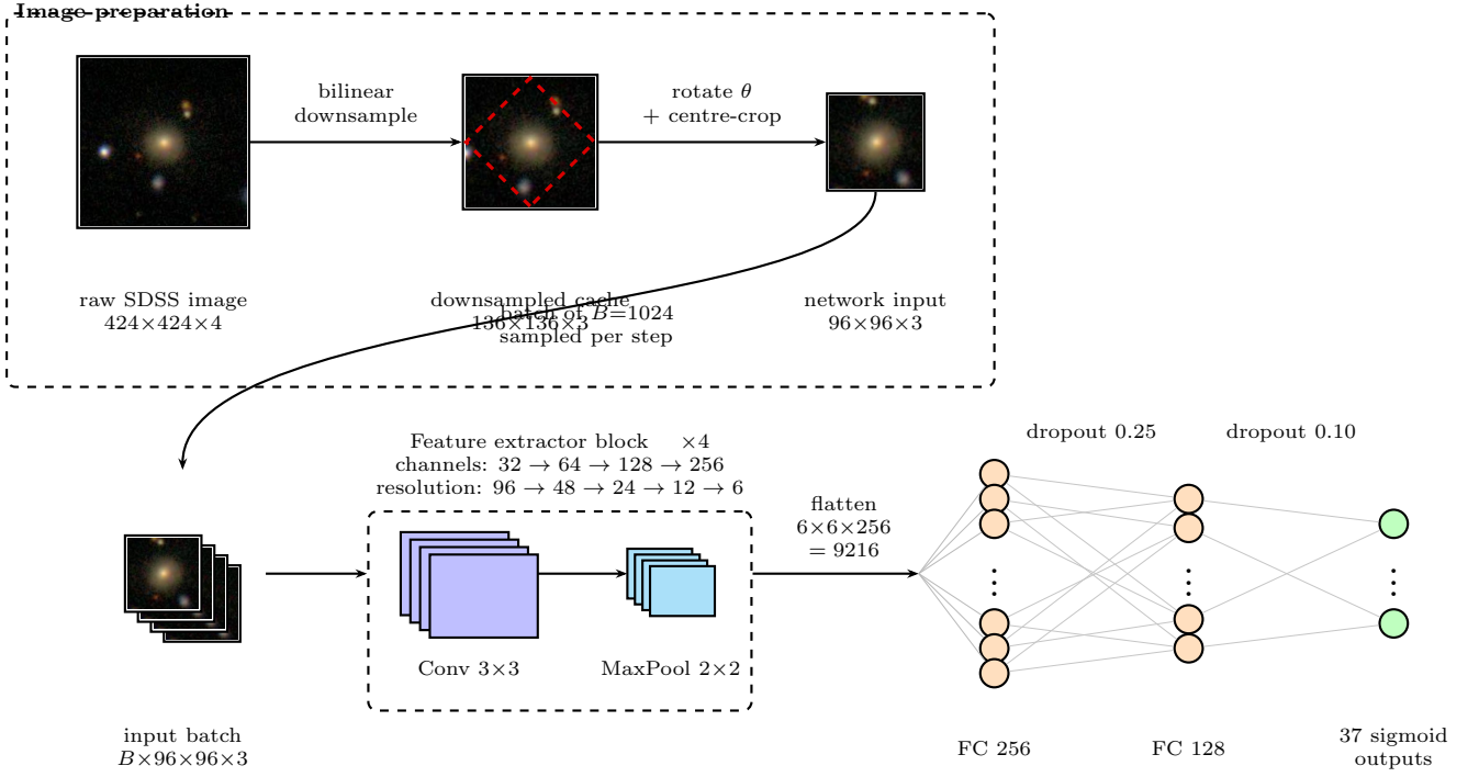
Fig. 18.— Custom CNN architecture, read top-to-bottom then left-to-right. Top row, image preparation: the raw 424^2 SDSS gri cutout is bilinearly downsampled to a 136^2 on-disk cache; the dashed red square inside the cache marks the rotated 96^2 crop region for one realisation of the augmentation angle \theta \in [0, 360^\circ) . The crop is then resampled to the upright 96^2 network input on the right — the rotation lives in the cache stage so the final input array stored on the GPU is always an axis-aligned square. The cache side 136 \geq 96\sqrt{2} guarantees the rotated crop region fits inside the cache at every angle, so no black corners ever enter the network (Section 3.4). Bottom row, Custom CNN ( \sim 2.8M params): batches of B = 1024 upright 96^2 \times 3 inputs pass through a feature extractor consisting of a 3 \times 3 convolution followed by 2 \times 2 max-pooling, with the dashed loop indicating the block is repeated four times at channel widths 32 \rightarrow 64 \rightarrow 128 \rightarrow 256 . The flattened feature vector is fully connected to 256 units, halved to 128 units, and finally projected onto 37 sigmoid outputs; dropout fractions 0.25 and 0.10 are applied to the two FC bundles, drawn schematically.
