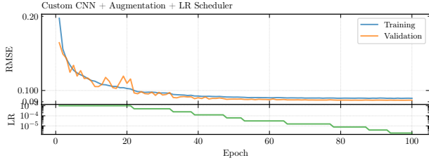
Fig. 25.— Custom CNN with rotation augmentation and the ReduceLROnPlateau scheduler (100 epochs). Best validation RMSE: 0.0913 at epoch 97, below the lab manual’s “good” target of 0.09 and the best result across all our trained models. The training curve is no longer monotonic (it wobbles in a band) because the optimiser sees a different rotation of each galaxy at every epoch; this is the signature that the model is learning rotation-invariant features rather than memorising the training set.
