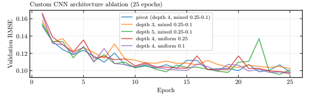
Fig. 21.— Architecture ablation: per-variant validation loss for the 5 architecture variants on the depth and dropout axes, each trained for 25 epochs from scratch. Depths 3, 4, 5 cluster within run-to-run noise; the tapered-dropout (0.25, 0.10) pivot is empirically justified over both uniform-dropout endpoints, motivating the (depth-4, tapered-dropout) configuration carried into the 100-epoch run.
