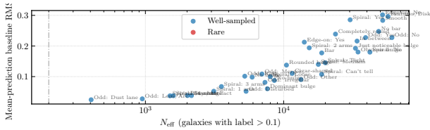
Fig. 10.— Effective sample size per label. Hierarchical gating drives deeper-tree labels to N_{\text{eff}} far below the nominal 61,578.
