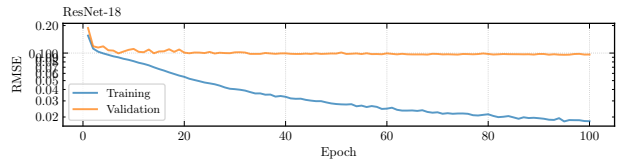
Fig. 20.— ResNet-18 training and validation RMSE vs. epoch (100 epochs, Adam, no augmentation, no scheduler). The best validation RMSE is 0.0958, reached at epoch 95. The training/validation gap grows visibly after epoch \sim 10 , the canonical signature of overfitting; the LR scheduler and rotation augmentation introduced in Section 4.4 close this gap. This figure is the Checkpoint 2 deliverable from the lab manual.
