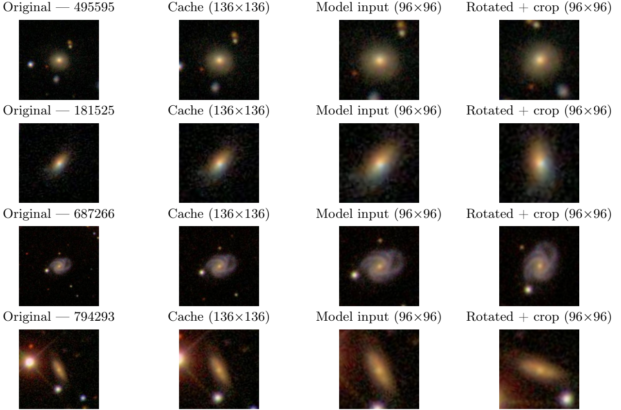
Fig. 16.— Pipeline stages for four example galaxies (rows): raw 424^2 SDSS GZ2 cutout, 136^2 rotation-safe cache, 96^2 centre-cropped model input, and one realisation of the same image after a random rotation by \theta \in [0, 360^\circ) . The rotated image always covers the centre 96^2 region with no black corner artefacts because the cache size 136 \geq 96\sqrt{2} is the smallest integer guaranteeing rotation-safety; this geometric constraint is the upstream design decision that makes the rotation-augmentation strategy of Section 4.4 defensible (no boundary artefacts ever enter the network’s training distribution).
