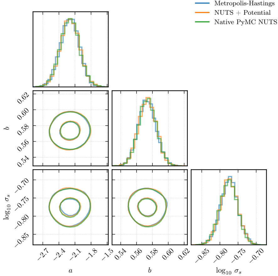
Fig. 17.— Overlay corner plot comparing all three MCMC methods for RRc : M-H (blue), NUTS+Potential (orange), native PyMC (green). The RRc posteriors are broader than R Rab (fewer stars), but all three methods converge to consistent posteriors.
