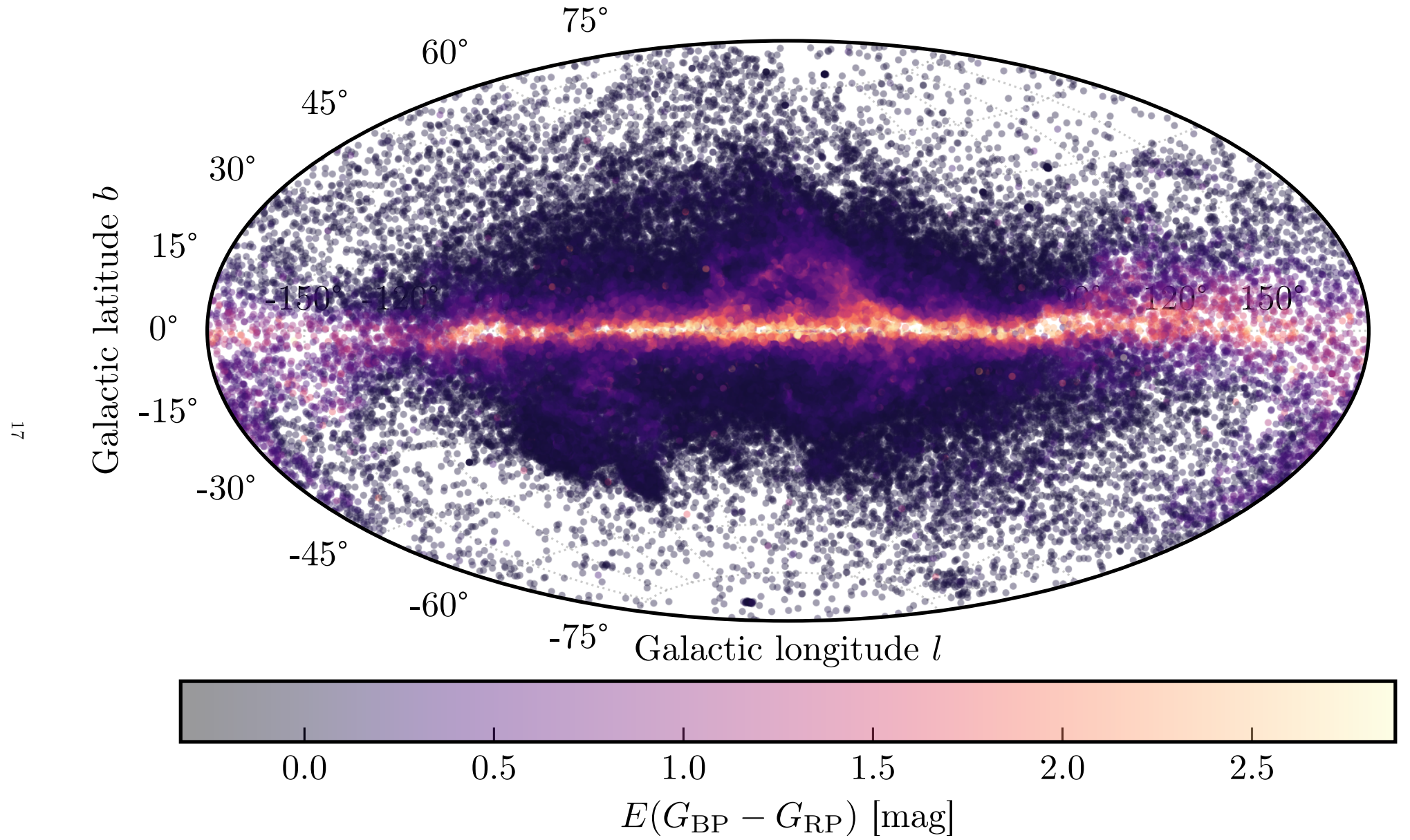
Fig. 21.— All-sky reddening map from 130,877 RR Lyrae stars (88,028 RRab + 42,849 RRC) in Aitoff (equal-area) projection. Color indicates E(G_{\text{BP}} - G_{\text{RP}}) in magnitudes. The Galactic plane shows high reddening; the Galactic center region (right) has the highest extinction. High-latitude regions show low, patchy reddening from nearby dust clouds; the Large and Small Magellanic Clouds appear clearly as overdensities. The non-uniform sky coverage reflects the non-uniform distribution of RR Lyrae stars.
