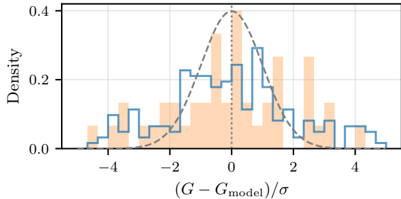
Best K = 5
