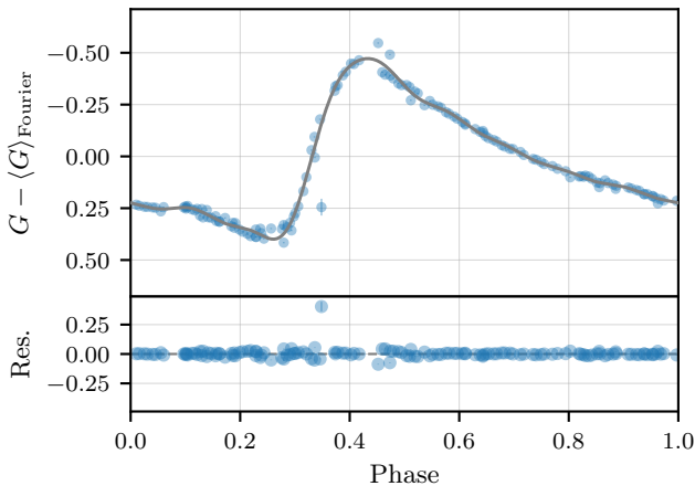
RRab: Gaia DR3 5283631727741891072 P = 0.6905 d, K = 9 , \chi^2_\nu = 43.51
