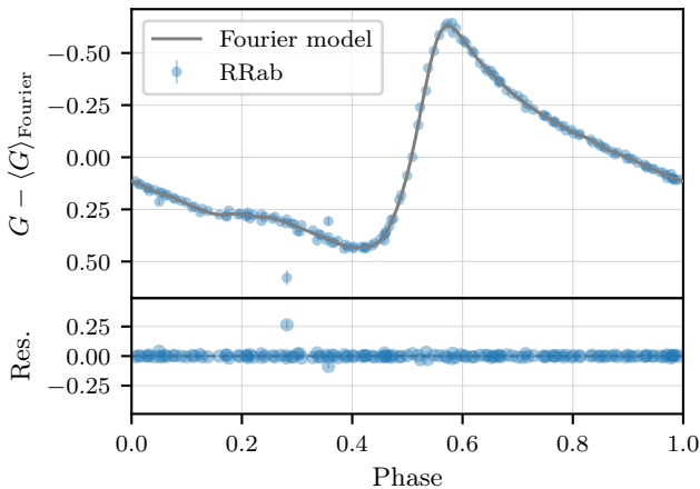
RRab: Gaia DR3 5283265044923053952 P = 0.6106 d, K = 17 , \chi^2_\nu = 11.99
