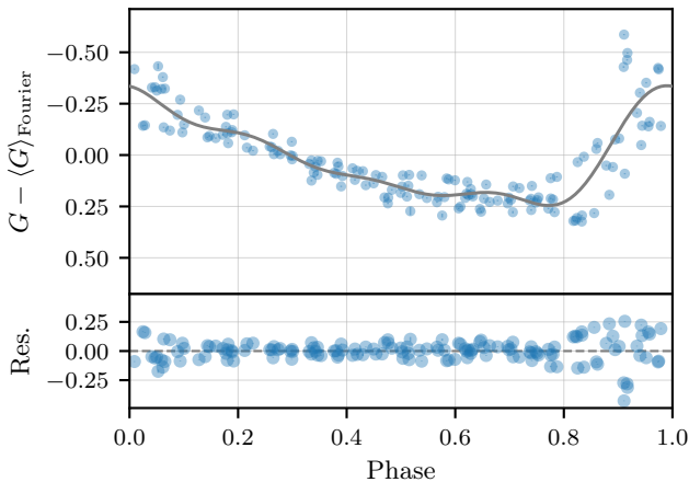
RRab: Gaia DR3 1275030757727244032 P = 0.5678 d, K = 4 , \chi^2_\nu = 857.38
