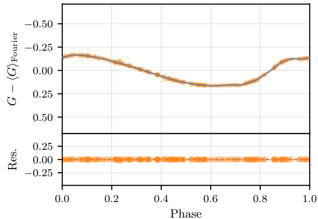
RRc: Gaia DR3 5873907641856894208 P = 0.2245 d, K = 17 , \chi^2_\nu = 1.43
