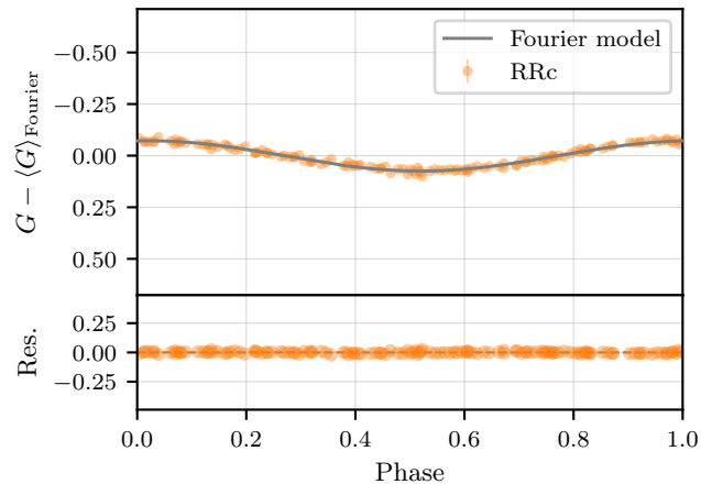
RRc: Gaia DR3 1634267186780543104 P = 0.2972 d, K = 1 , \chi^2_\nu = 6.31
