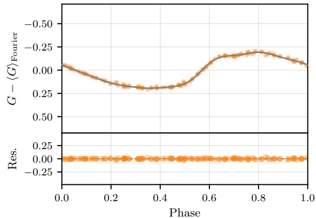
RRc: Gaia DR3 6434006595919847040 P = 0.2370 d, K = 6 , \chi^2_\nu = 6.25
