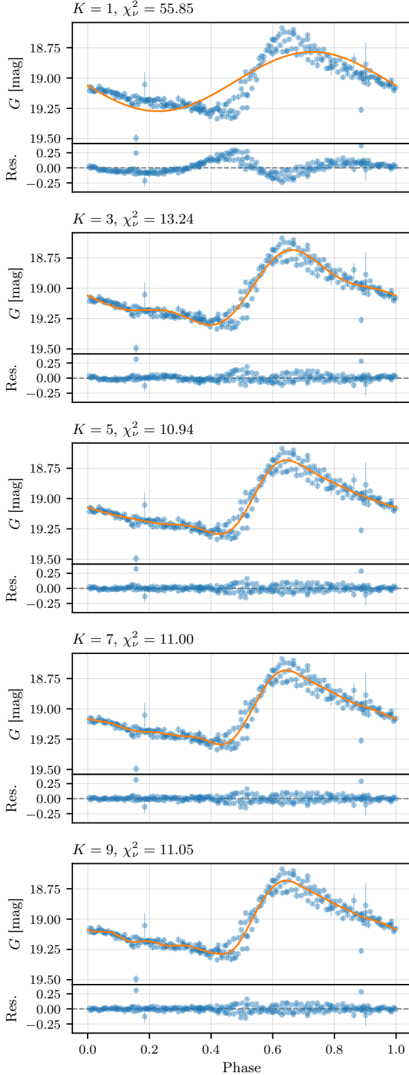
Fig. 5.— Fourier series fits of order K = 1, 3, 5, 7, 9 to the phase-folded RRab light curve. Low orders ( K = 1, 3 ) fail to capture the rapid rise; K = 5 provides a good fit; higher orders begin to overfit noise.
