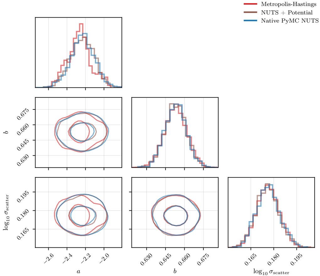
Fig. 15.— Overlay corner plot comparing all three MCMC methods for RRab : M-H (red), NUTS+Potential (brown), native PyMC (blue). All three converge to consistent posteriors, validating our implementation.
