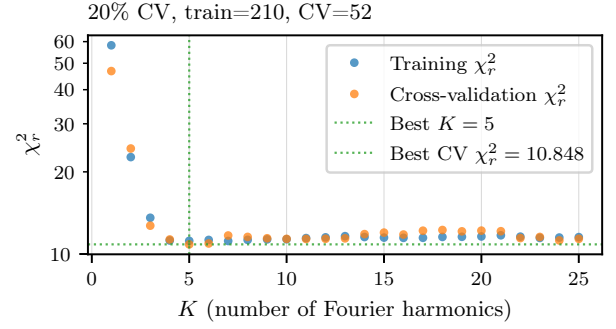
Fig. 6.— Cross-validation curve for the example RRab star where training \chi_r^2 (blue) and validation \chi_r^2 (orange) as a function of Fourier order K . The optimal K = 5 minimizes validation error before overfitting sets in.
