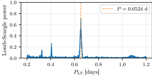
Fig. 3.— Lomb-Scargle periodogram for the star shown in Figure 2. The vertical dashed line marks the peak period P_{\text{LS}} adopted for subsequent Fourier fitting.
