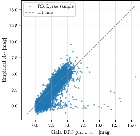
Fig. 19.— Empirical A_G (this work) vs. Gaia DR3 g_{\text{absorption}} for 109,325 RRAb stars with finite Gaia extinction estimates. The dashed line shows the 1:1 relation.
