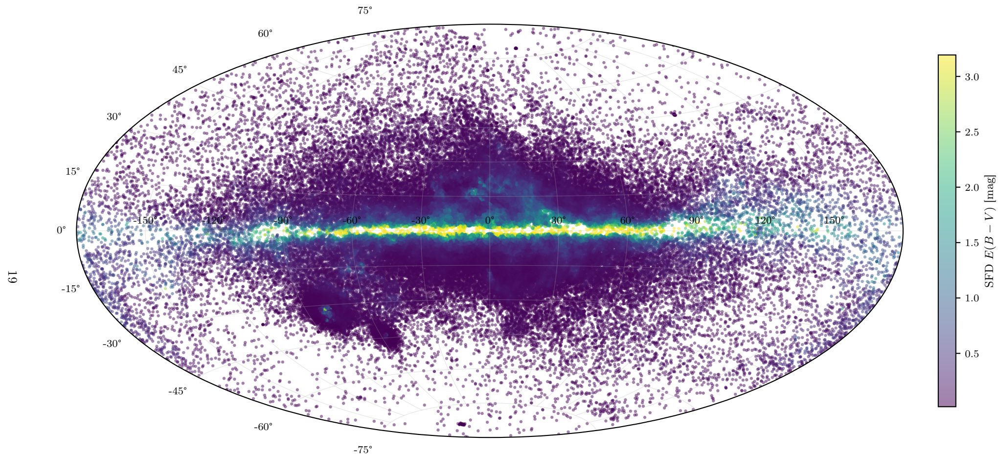
Fig. 21.— SFD E(B-V) (Schlegel et al. 1998) sampled at the sky positions of the 130,877 cleaned RR Lyrae stars in Aitoff (equal-area) projection. The map traces the total dust column integrated to infinity along each sightline; compare with Figure 20, which shows only the foreground dust out to each star’s heliocentric distance. The Galactic plane and center show markedly higher E(B-V) in SFD than in the empirical RR Lyrae map which provides direct evidence of the 3D vs. 2D effect explored quantitatively in Section 9.6.
