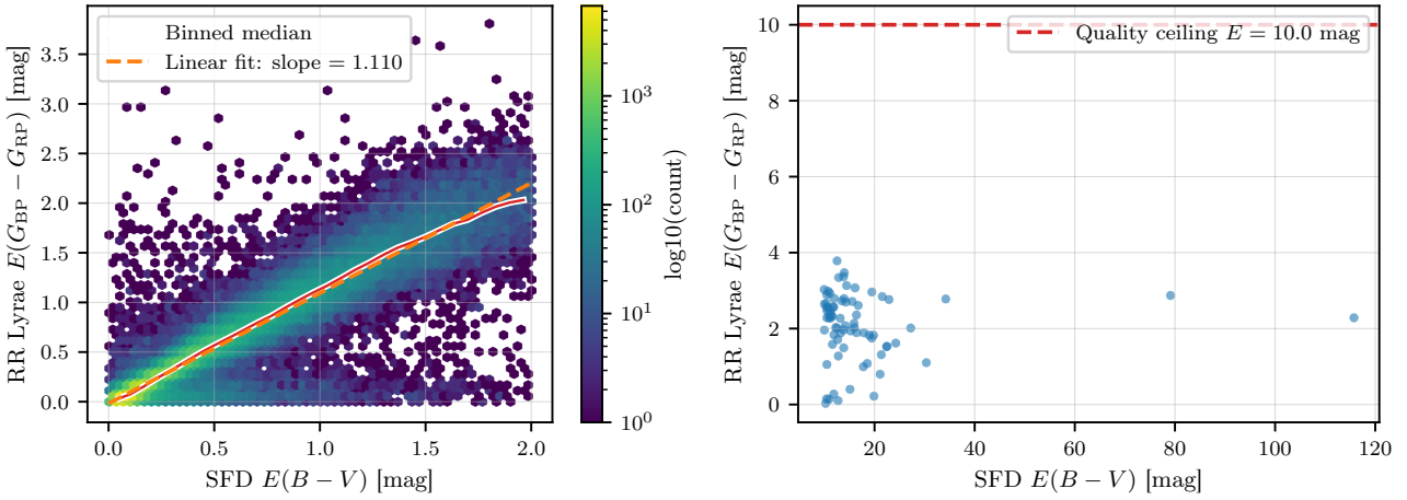
Fig. 22.— Regime decomposition of the SFD vs. empirical comparison. Left : Similar-scale regime ( E(B - V)_{\text{SFD}} \leq 2 mag, N = 127,893 stars). The density hexbin shows a tight linear trend; the dashed orange line is a linear fit with slope 1.11, below the expected Gaia-band conversion factor R_{BP-RP} \approx 1.3 . Right : Large-SFD regime ( E(B - V)_{\text{SFD}} > 10 mag, N = 74 stars). The empirical E(G_{\text{BP}} - G_{\text{RP}}) saturates far below the SFD column despite the physical ceiling at 10.0 mag being well above the observed values. The decoupling illustrates the 3D vs. 2D distinction between a distance-limited stellar measurement and a total-column dust map.
