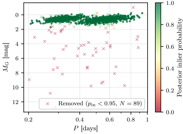
Fig. 14.— G -band period–absolute magnitude diagram color-coded by posterior inlier probability. Circles show retained stars ( p_{\text{in}} \geq 0.95 ); crosses mark the flagged outliers ( p_{\text{in}} < 0.95 ) removed from the calibration sample.
