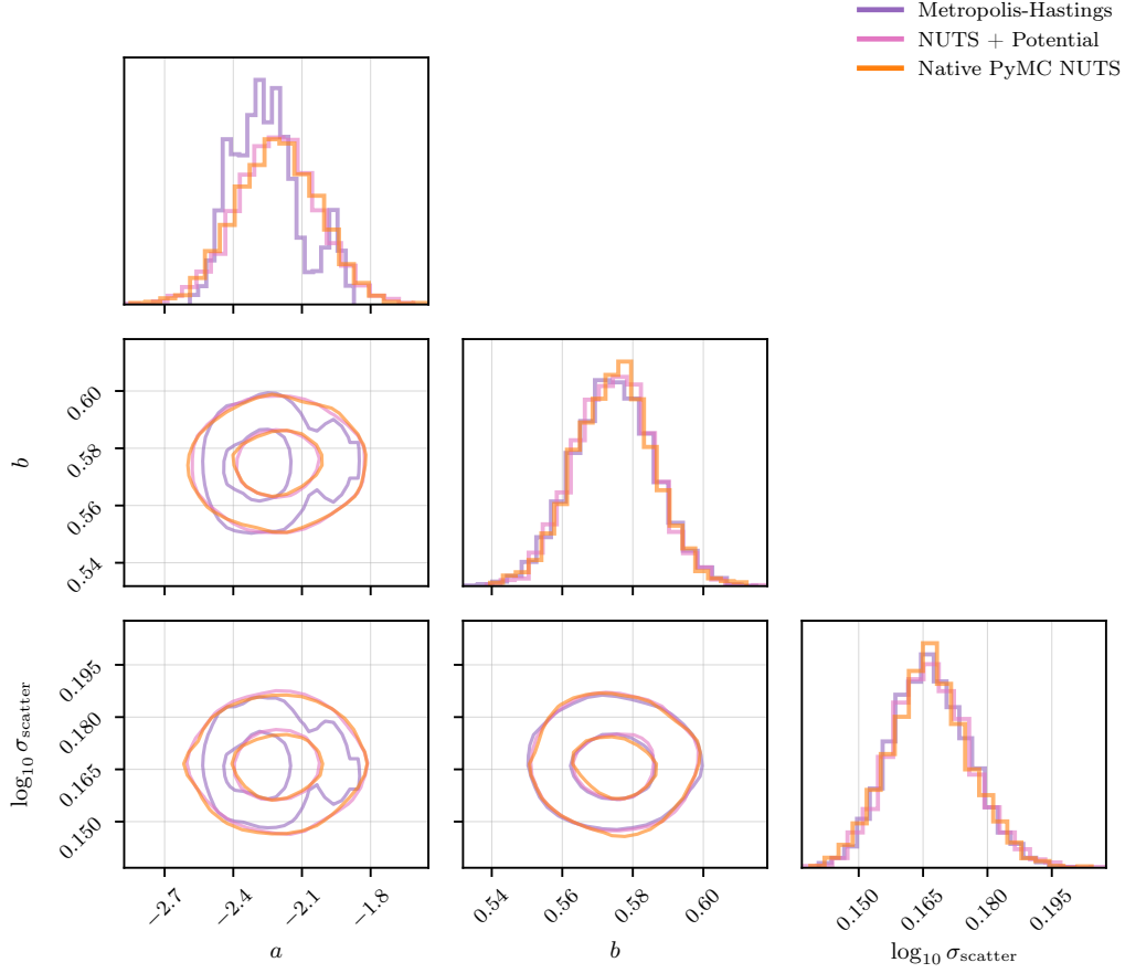
Fig. 16.— Overlay corner plot comparing all three MCMC methods for RRc : M-H (purple), NUTS+Potential (pink), native PyMC (orange). The RRc posteriors are broader than RRab (fewer stars), but all three methods converge to consistent posteriors.
