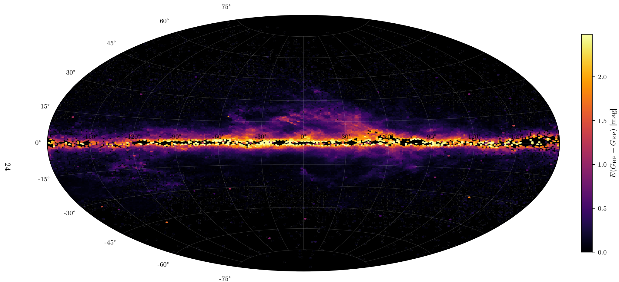
Fig. 23.— A cooler looking all-sky reddening map rendered on a black background using the inferno colorscale, mapping zero reddening to black and increasing dust columns to progressively brighter orange and yellow. Same 130,877 stars as Figure 20. The dark background suppresses empty sky and makes the filamentary structure of nearby dust clouds and the Galactic warp visually prominent.
