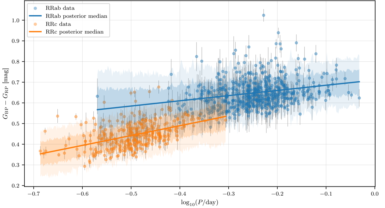
Fig. 18.— Joint period-color posterior predictive comparison for RRAb (blue) and RRc (orange) in the same coordinate system. The RRc slope ( a_{c,RRc} = +0.48 \pm 0.05 ) is roughly twice as steep as the RRAb slope ( a_{c,RRab} = +0.25 \pm 0.04 ), confirming stronger temperature-period coupling in first-overtone pulsators.
