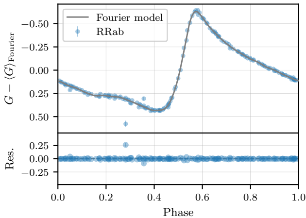
RRab: Gaia DR3 1275030757727244032 P = 0.5678 d, K = 4 , \chi^2_\nu = 857.38
