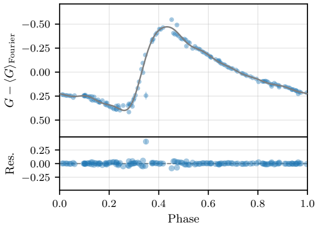
RRab: Gaia DR3 5283631727741891072 P = 0.6905 d, K = 9 , \chi^2_\nu = 43.51
