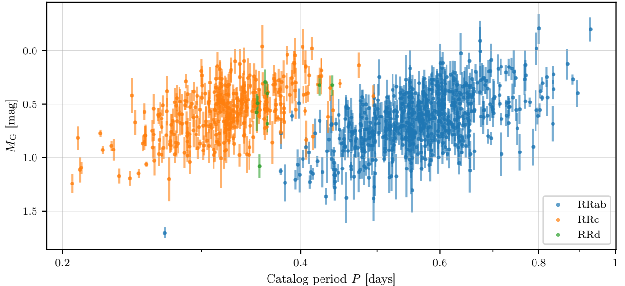
Fig. 15.— G -band period–absolute magnitude diagram for the final cleaned calibration sample ( N = 884 ) after mixture contamination model rejection ( p_{\text{in}} \geq 0.95 ). Points are colored by pulsation subclass (RRab, RRc, RRd). Error bars show combined photometric and parallax uncertainties.
