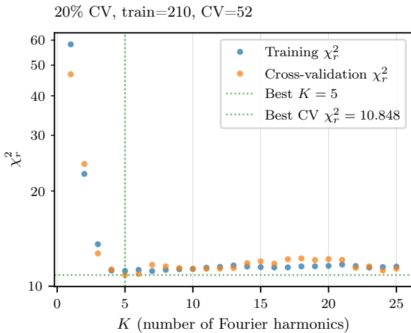
Fig. 6.— Cross-validation curve for the example RRab star where training \chi_r^2 (blue) and validation \chi_r^2 (orange) as a function of Fourier order K . The optimal K = 5 minimizes validation error before overfitting sets in.
