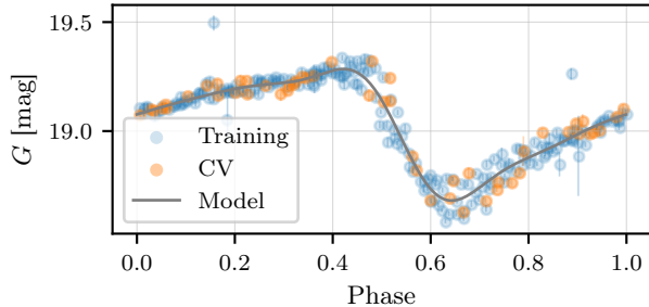
Best K = 5
