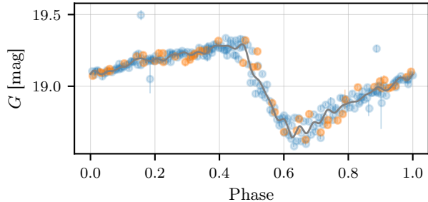
High K = 25
