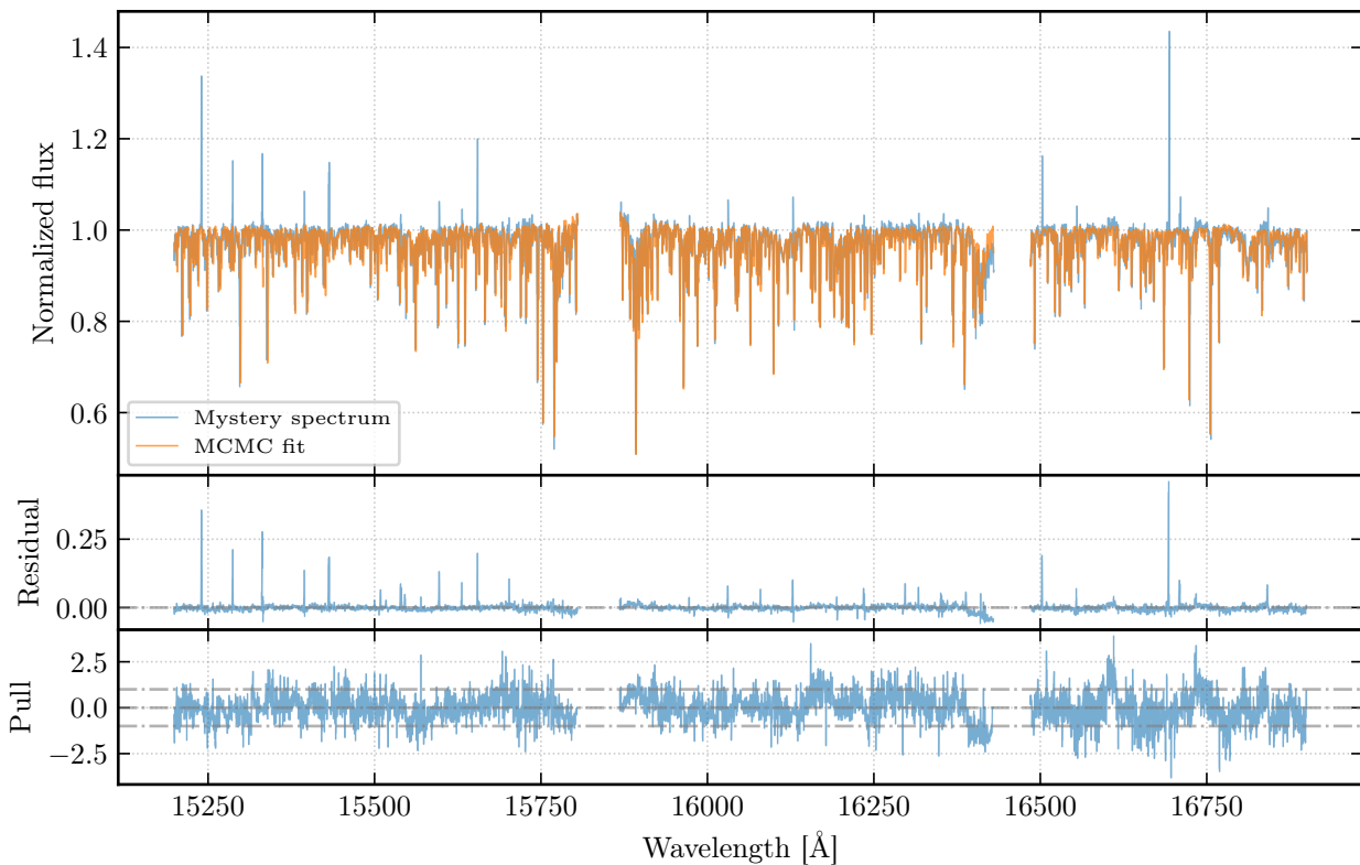
Mystery spectrum, 15200–16900 Å
