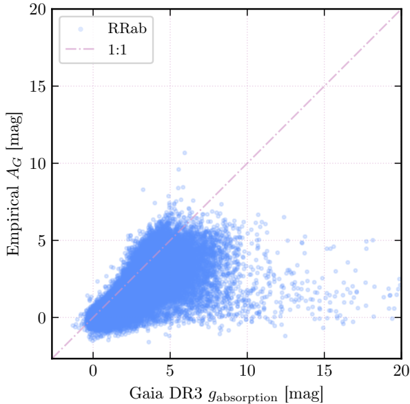
Fig. 20.— Empirical A_G (this work) vs. Gaia DR3 g -absorption for 109,325 RRab stars with finite Gaia extinction estimates. The dashed line shows the 1:1 relation.
