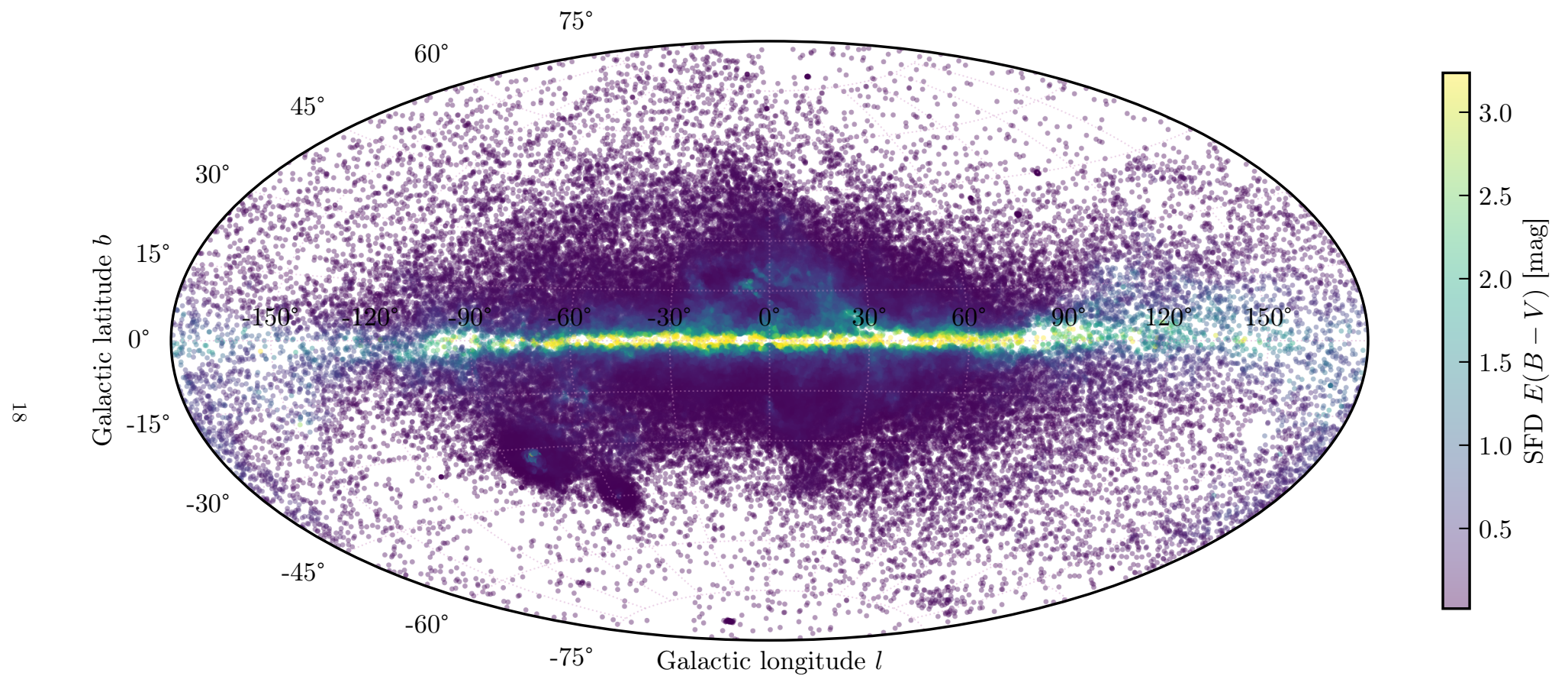
Fig. 22.— SFD E(B - V) (?) sampled at the sky positions of the 130,877 cleaned RR Lyrae stars in Aitoff (equal-area) projection. The map traces the total dust column integrated to infinity along each sightline; compare with Figure ??, which shows only the foreground dust out to each star's heliocentric distance. The Galactic plane and center show markedly higher E(B - V) in SFD than in the empirical RR Lyrae map which provides direct evidence of the 3D vs. 2D effect explored quantitatively in Section ??.
