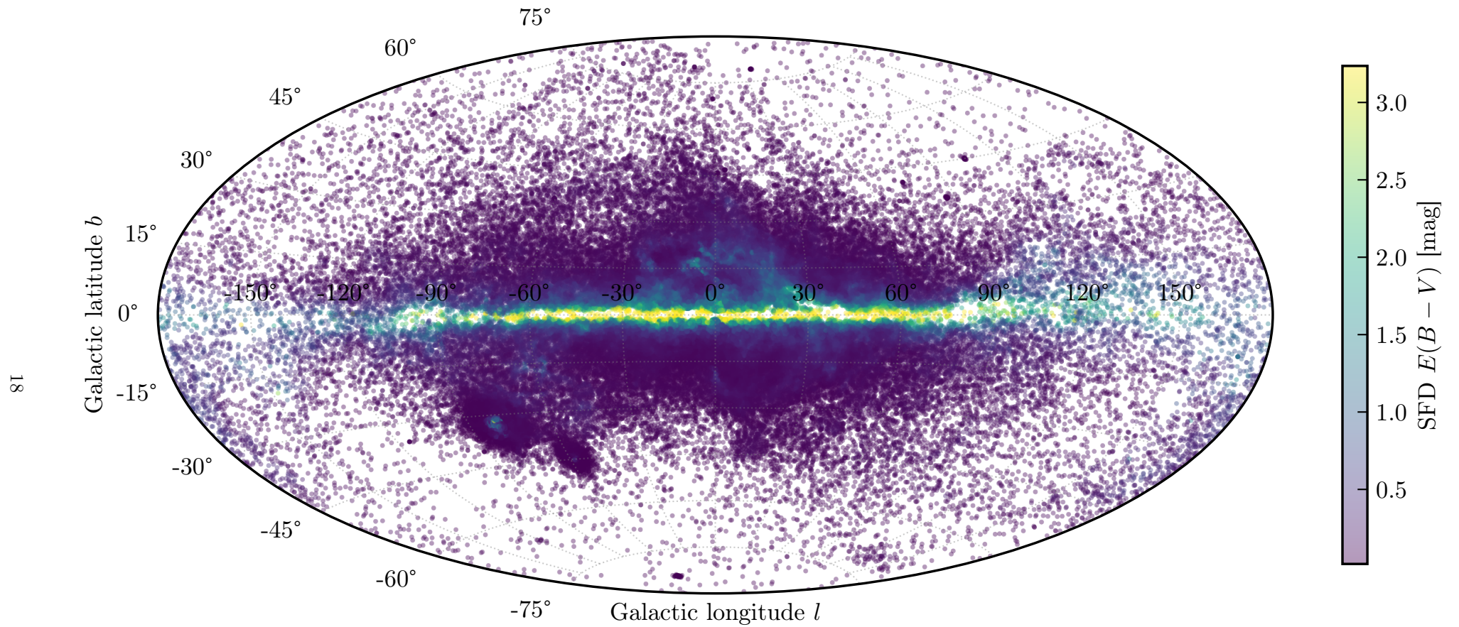
Fig. 22.— SFD E(B - V) (D. J. Schlegel et al. 1998) sampled at the sky positions of the 131,213 cleaned RR Lyrae stars in Aitoff (equal-area) projection. The map traces the total dust column integrated to infinity along each sightline; compare with Figure 21, which shows only the foreground dust out to each star’s heliocentric distance. The Galactic plane and center show markedly higher E(B - V) in SFD than in the empirical RR Lyrae map which provides direct evidence of the 3D vs. 2D effect explored quantitatively in Section 9.6.
