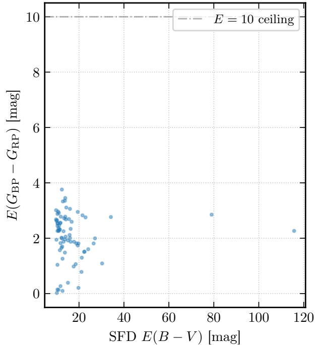
Fig. 23.— Regime decomposition of the SFD vs. empirical comparison. Left : Similar-scale regime ( E(B - V)_{\text{SFD}} \leq 2 mag, N = 128,154 stars). The density hexbin shows a tight linear trend; the dashed orange line is a linear fit with slope 1.11, below the expected Gaia-band conversion factor R_{BP-RP} \approx 1.3 . Right : Large-SFD regime ( E(B - V)_{\text{SFD}} > 10 mag, N = 77 stars). The empirical E(G_{BP} - G_{RP}) saturates far below the SFD column despite the physical ceiling at 10.0 mag being well above the observed values. The decoupling illustrates the 3D vs. 2D distinction between a distance-limited stellar measurement and a total-column dust map.
