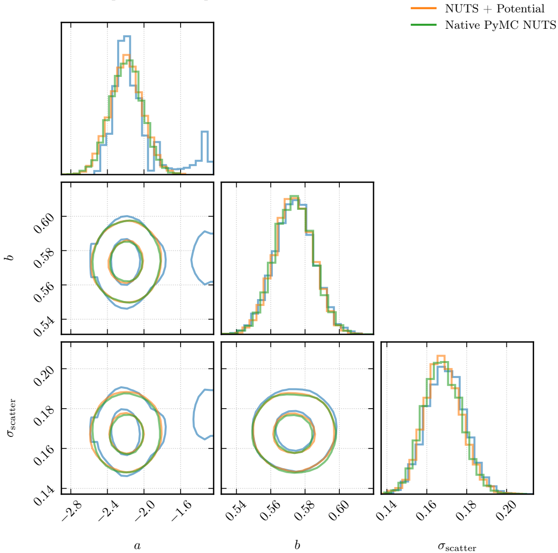
RRc: posterior comparison across all three MCMC methods
