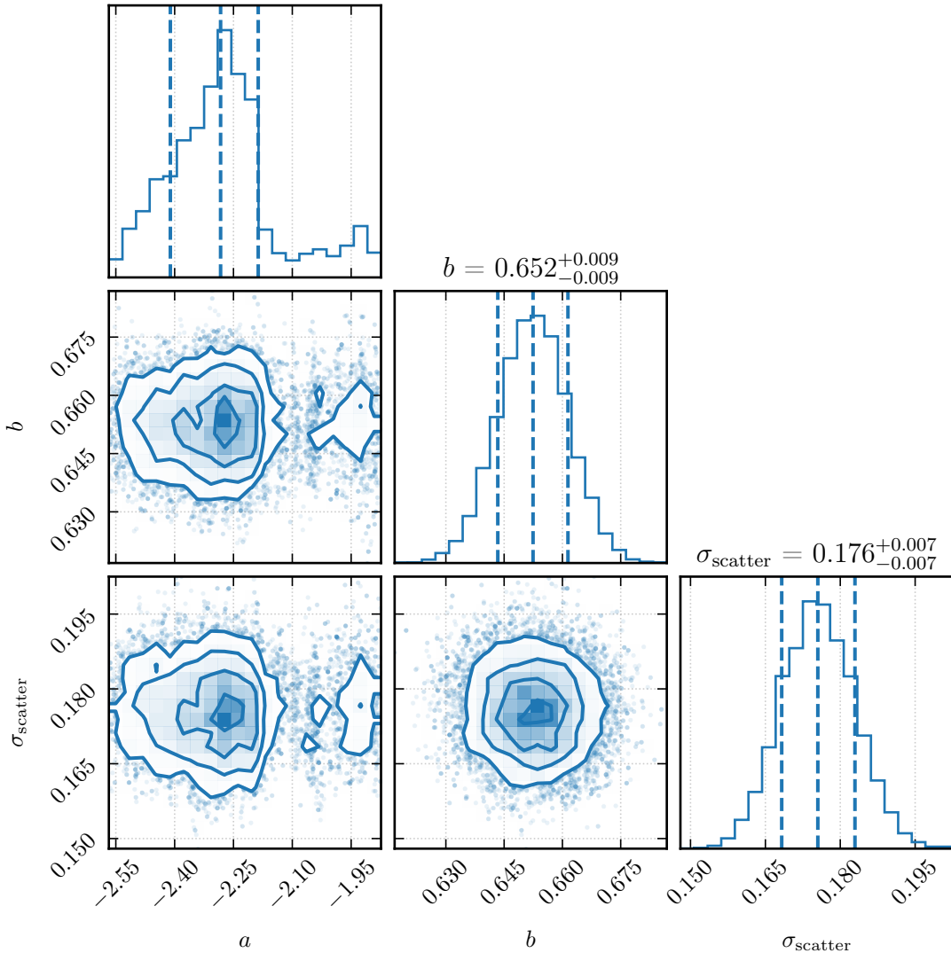
Posterior Distributions of a , b , and \sigma_{\text{scatter}} (Metropolis-Hastings)
