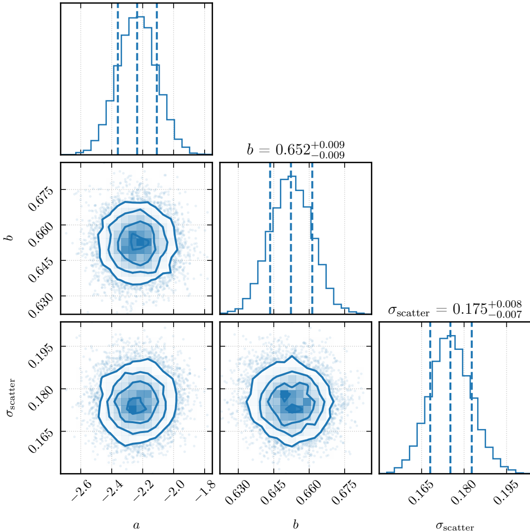
Posterior distributions of a , b , and \sigma_{\text{scatter}} (native PyMC NUTS)
