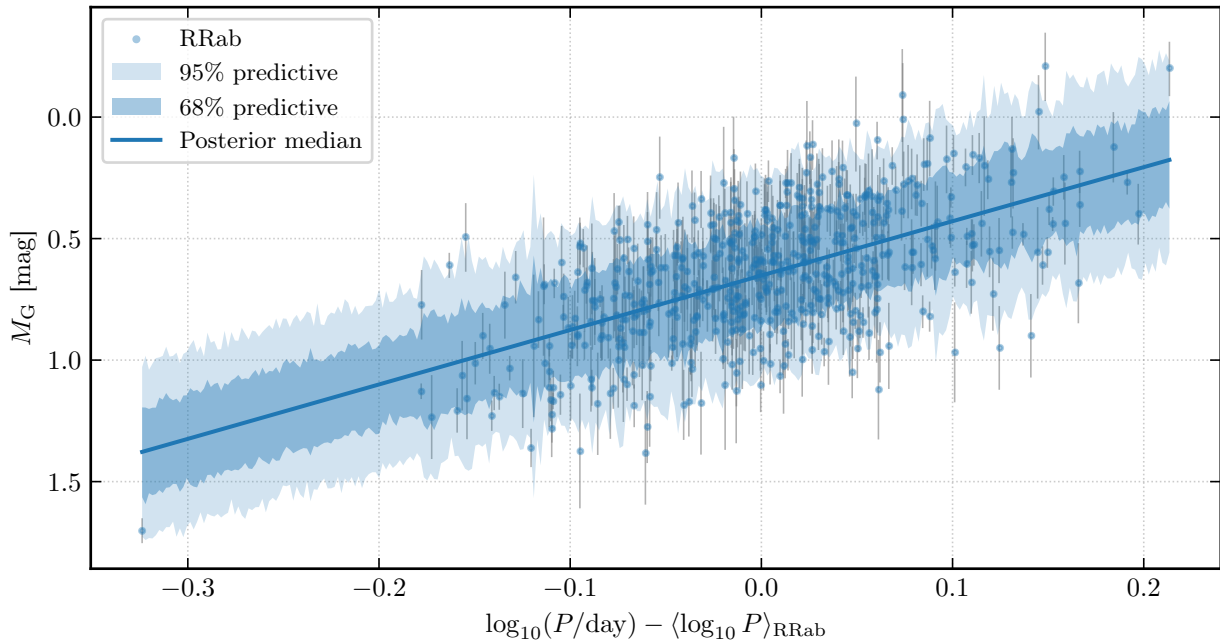
RRab posterior predictive check (native PyMC NUTS)
