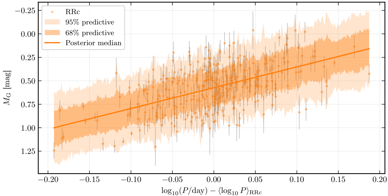
RRc posterior predictive check (native PyMC NUTS)
