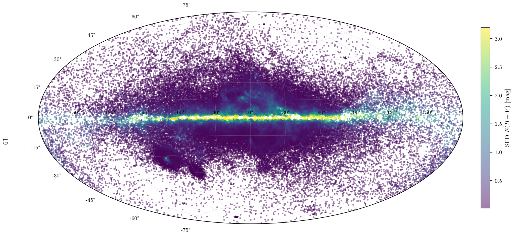
Fig. 22.— SFD E(B - V) (Schlegel et al. 1998) sampled at the sky positions of the 130,877 cleaned RR Lyrae stars in Aitoff (equal-area) projection. The map traces the total dust column integrated to infinity along each sightline; compare with Figure 21, which shows only the foreground dust out to each star’s heliocentric distance. The Galactic plane and center show markedly higher E(B - V) in SFD than in the empirical RR Lyrae map which provides direct evidence of the 3D vs. 2D effect explored quantitatively in Section 9.6.
