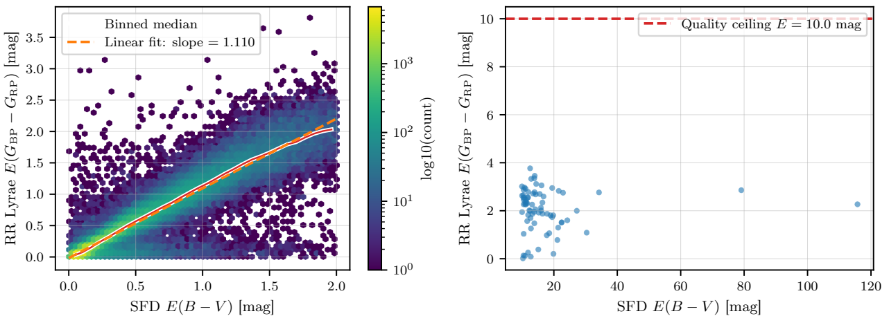
Fig. 23.— Regime decomposition of the SFD vs. empirical comparison. Left : Similar-scale regime ( E(B - V)_{\text{SFD}} \leq 2 mag, N = 127,893 stars). The density hexbin shows a tight linear trend; the dashed orange line is a linear fit with slope 1.11, below the expected Gaia-band conversion factor R_{BP-RP} \approx 1.3 . Right : Large-SFD regime ( E(B - V)_{\text{SFD}} > 10 mag, N = 74 stars). The empirical E(G_{BP} - G_{RP}) saturates far below the SFD column despite the physical ceiling at 10.0 mag being well above the observed values. The decoupling illustrates the 3D vs. 2D distinction between a distance-limited stellar measurement and a total-column dust map.
