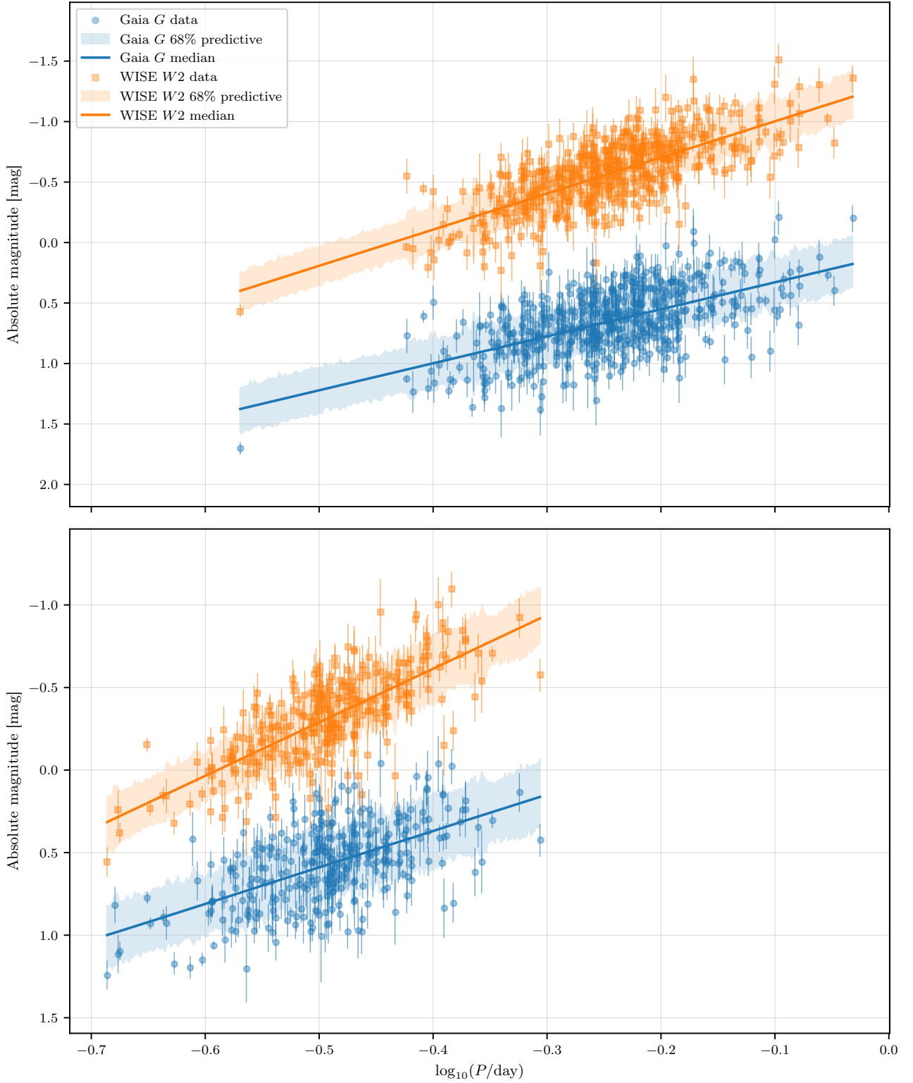
Fig. 18.— Side-by-side comparison of the Gaia G -band (blue) and WISE W2 (orange) period-luminosity relations for RRab ( top ) and RRc ( bottom ). Shaded bands show 68% posterior predictive envelopes. The steeper W2 slope ( \Delta a_{\text{RRab}} = -0.75 \pm 0.17 , \Delta a_{\text{RRc}} = -1.03 \pm 0.24 ) is visible as a more pronounced tilt in the orange fit lines relative to the blue. The tighter W2 scatter also reflects reduced extinction sensitivity at mid-infrared wavelengths.
