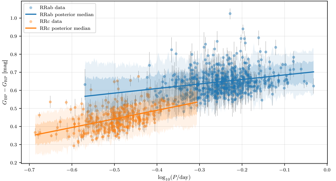
Fig. 19.— Joint period-color posterior predictive comparison for RRab (blue) and RRc (orange) in the same coordinate system. The RRc slope ( a_{c,\text{RRc}} = +0.48 \pm 0.05 ) is roughly twice as steep as the RRab slope ( a_{c,\text{RRab}} = +0.25 \pm 0.04 ), confirming stronger temperature-period coupling in first-overtone pulsators.
