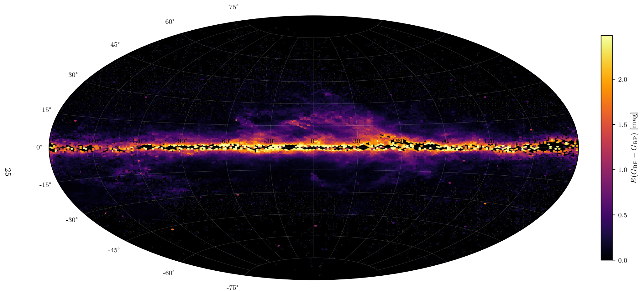
Fig. 24.— A cooler looking all-sky reddening map rendered on a black background using the inferno colorscale, mapping zero reddening to black and increasing dust columns to progressively brighter orange and yellow. Same 130,877 stars as Figure 21. The dark background suppresses empty sky and makes the filamentary structure of nearby dust clouds and the Galactic warp visually prominent.
