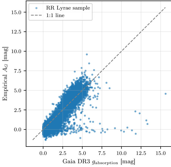
Fig. 20.— Empirical A_G (this work) vs. Gaia DR3 g_{\text{absorption}} for 109,325 RRab stars with finite Gaia extinction estimates. The dashed line shows the 1:1 relation.
