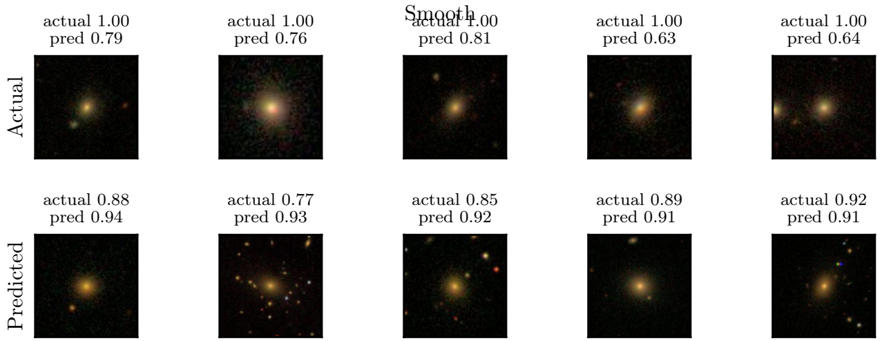
Fig. 19.— Top-5 images for “Smooth” by actual (top) and predicted (bottom) label.
