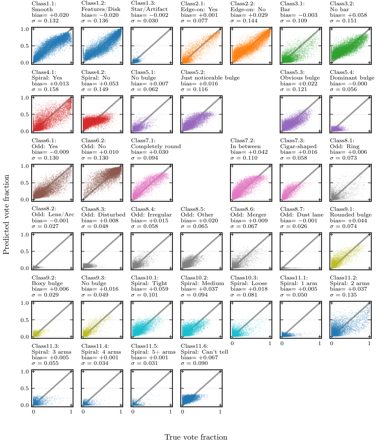
Fig. 18.— True vs. predicted vote fractions for all 37 GZ2 labels on the validation set, computed with the tree-weighted-loss Custom CNN. Panels are laid out by GZ2 decision-tree class and coloured by parent question; the diagonal is the 1:1 guide and per-panel bias and 1\sigma residual scatter are annotated.
