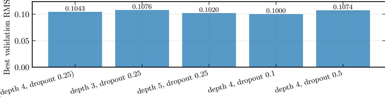
Custom CNN architecture ablation (15 epochs)
