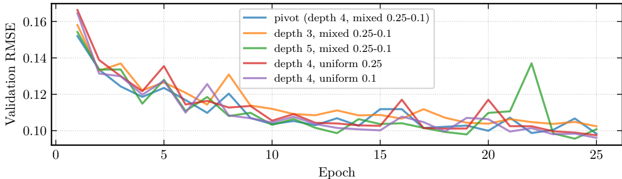
Custom CNN architecture ablation (25 epochs)
