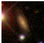
Cache (136×136)
