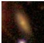
Model input (96×96)
