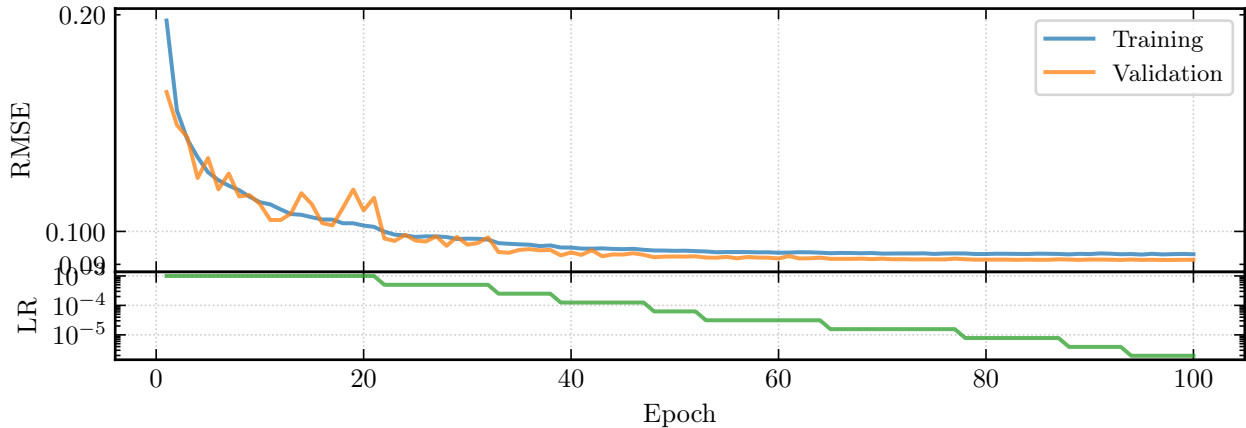
Custom CNN + Augmentation + LR Scheduler
