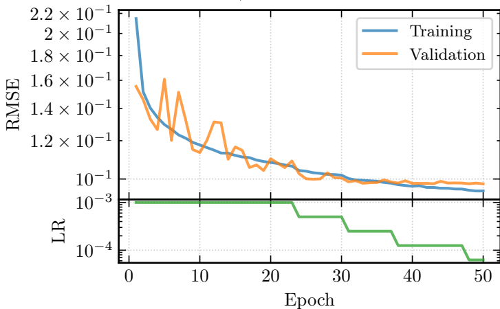
Custom CNN + LR Scheduler
