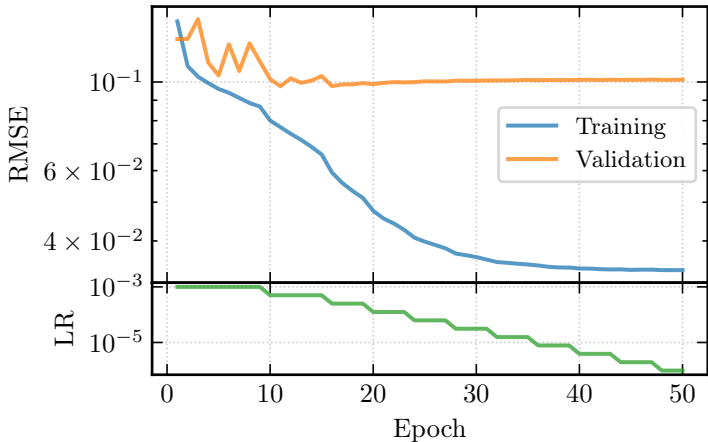
ResNet-18 + LR Scheduler
