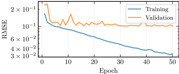
ResNet-18
