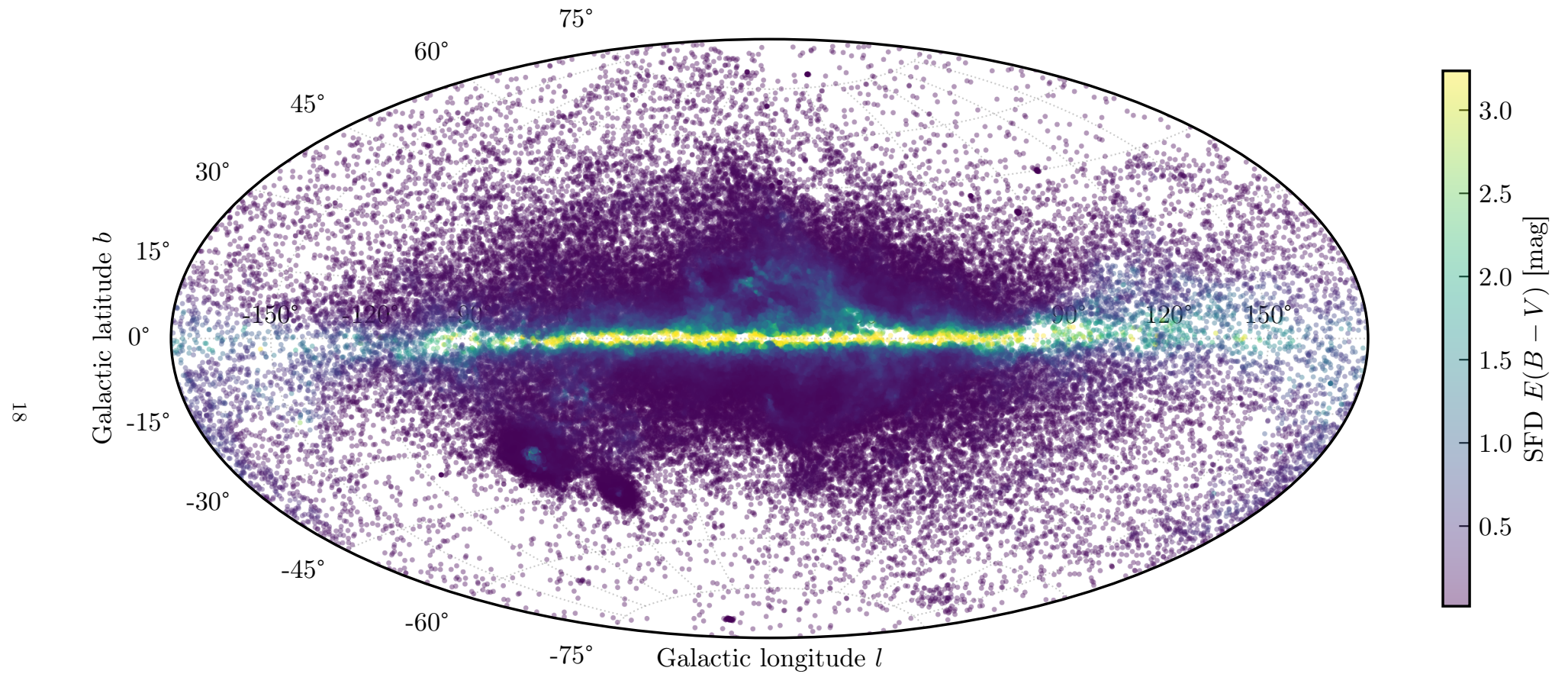
Fig. 22.— SFD E(B - V) (Schlegel et al. 1998) sampled at the sky positions of the 130,877 cleaned RR Lyrae stars in Aitoff (equal-area) projection. The map traces the total dust column integrated to infinity along each sightline; compare with Figure 21, which shows only the foreground dust out to each star’s heliocentric distance. The Galactic plane and center show markedly higher E(B - V) in SFD than in the empirical RR Lyrae map which provides direct evidence of the 3D vs. 2D effect explored quantitatively in Section 9.6.
