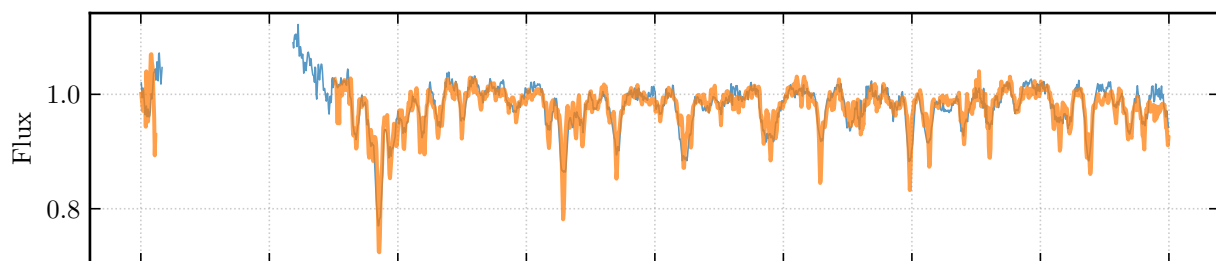
2M19403522+2411380
