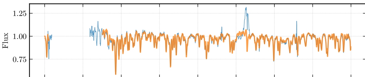
2M19464751+2354171
