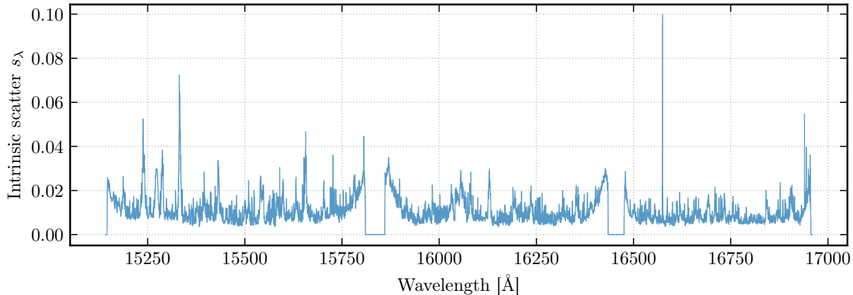
Per-pixel intrinsic scatter
