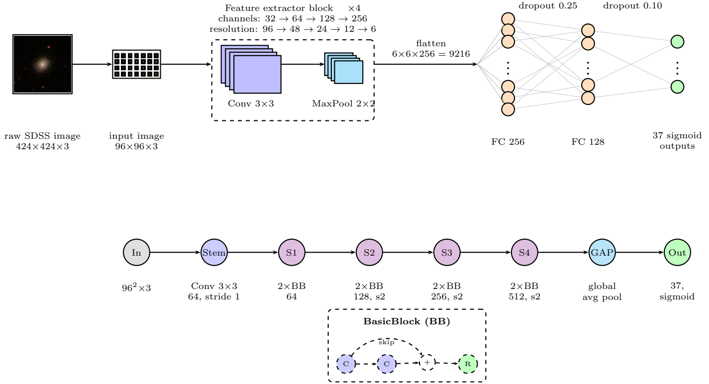
Fig. 17.— Architecture flow for the two backbones, read left-to-right. Top, Custom CNN ( \sim 2.8 M params): a 96 \times 96 \times 3 input image passes through a convolutional feature extractor consisting of a stack of 3 \times 3 convolutions followed by 2 \times 2 max-pooling, with the dashed loop indicating the block is repeated four times at channel widths 32 \rightarrow 64 \rightarrow 128 \rightarrow 256 . The flattened feature vector is then fully connected to 256 units, halved to 128 units, and finally projected onto 37 sigmoid outputs. Edges between FC layers are drawn schematically. Bottom, ResNet-18 ( \sim 11.2 M params): a 3 \times 3 /stride-1 stem (no initial max-pool, suitable for the small 96 \times 96 input) feeds four residual stages (S1–S4) of two BasicBlocks each at channel widths 64/128/256/512, ending in global average pooling and a 37-way sigmoid head. The dashed inset shows the internal flow of one BasicBlock: two 3 \times 3 convolutions (C) summed with the identity skip (+) followed by ReLU (R).
