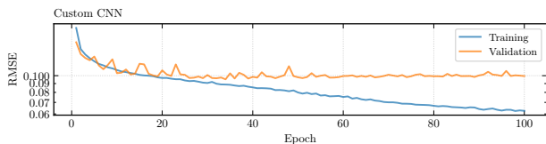
Fig. 20.— Custom CNN training and validation RMSE vs. epoch (100 epochs, Adam, no augmentation, no scheduler). The best validation RMSE is 0.0953, reached at epoch 34. The model is roughly 4\times smaller than ResNet-18 in parameter count but achieves a marginally lower bulk RMSE in this unaugmented baseline. The same train/val gap as in the ResNet baseline is visible.
