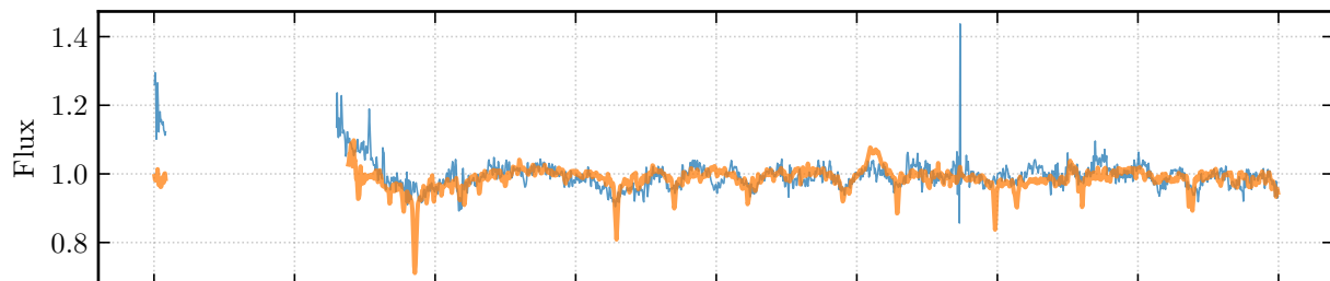
2M19445606+2411079
