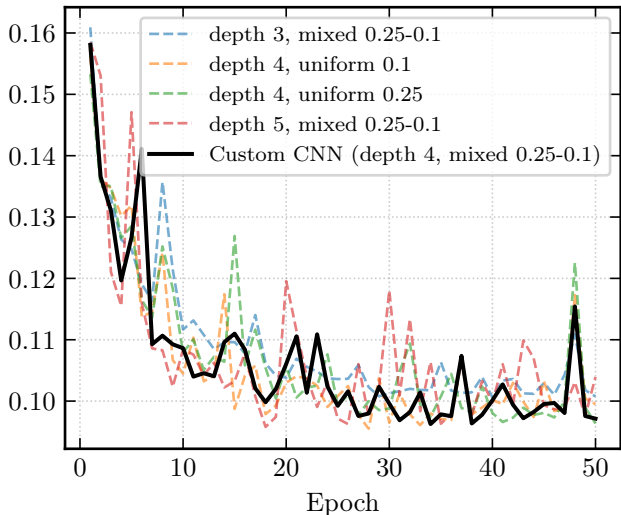
Validation RMSE
